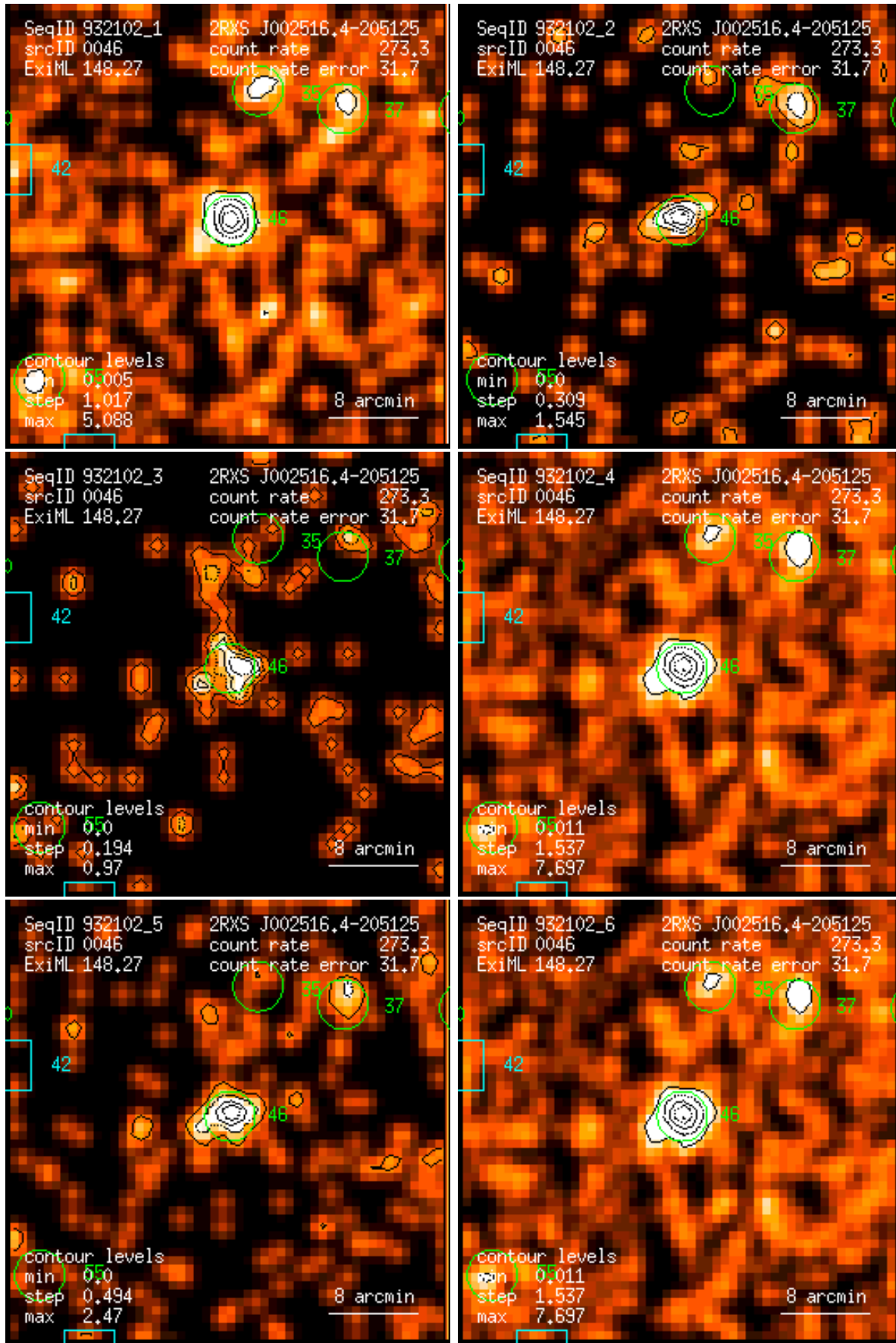
Figure 46: RASS 932102: detection 0046: band rate images, Gaussian filter: (1) PSPC channels 11 – 41, (2) 52 – 90, (3) 91 – 201, (4) 11 – 235, (5) 52 – 201, (6) 11 – 201. Broad band rates in counts/ks. Band rate contour levels in counts/ks/arcmin 2 .
