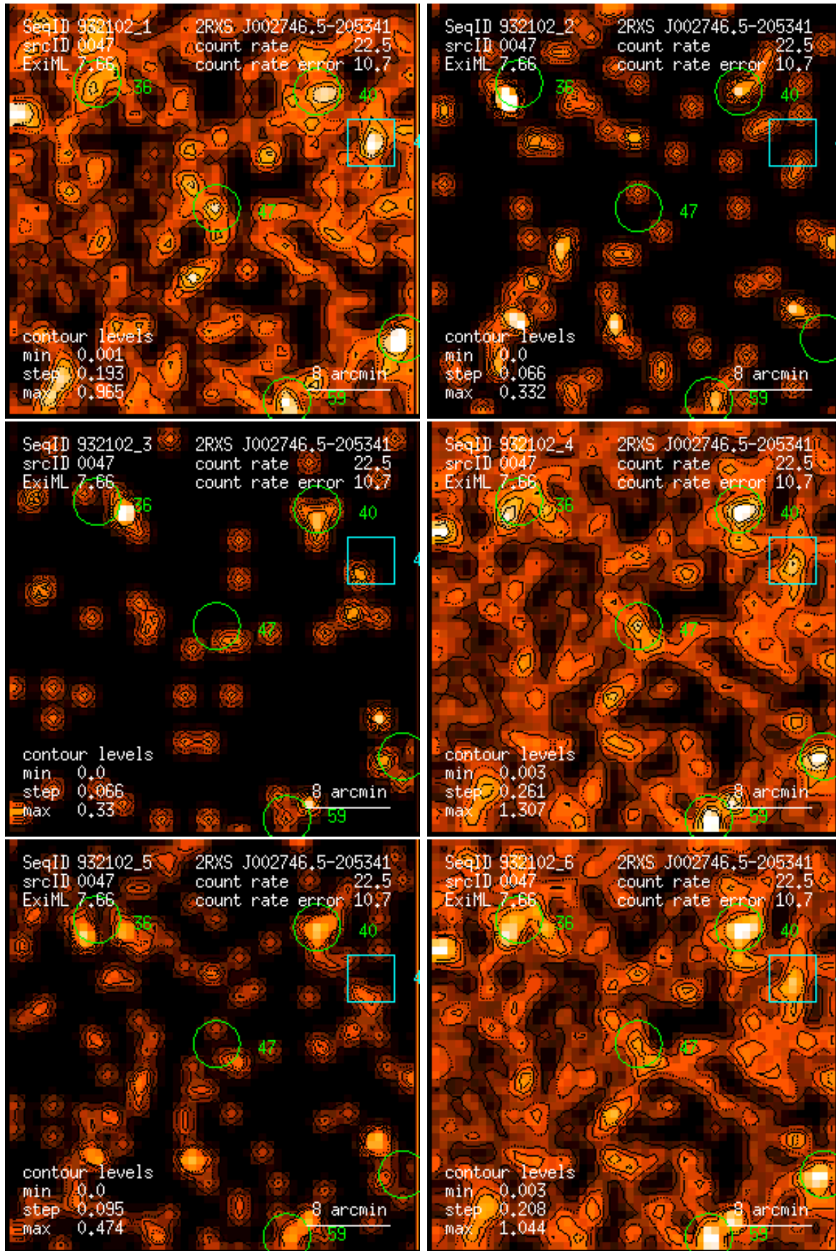
Figure 47: RASS 932102: detection 0047: band rate images, Gaussian filter: (1) PSPC channels 11 – 41, (2) 52 – 90, (3) 91 – 201, (4) 11 – 235, (5) 52 – 201, (6) 11 – 201. Broad band rates in counts/ks. Band rate contour levels in counts/ks/arcmin 2 .
