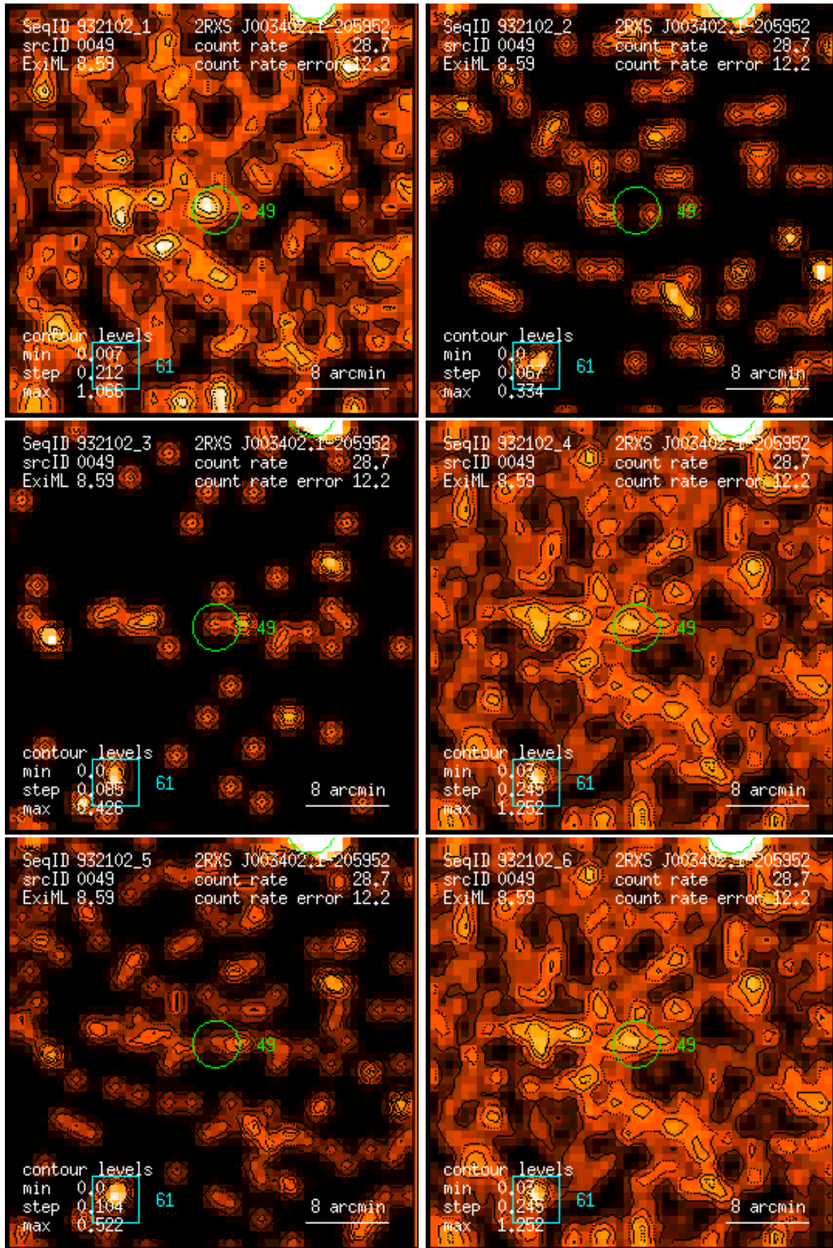
Figure 49: RASS 932102: detection 0049: band rate images, Gaussian filter: (1) PSPC channels 11 – 41, (2) 52 – 90, (3) 91 – 201, (4) 11 – 235, (5) 52 – 201, (6) 11 – 201. Broad band rates in counts/ks. Band rate contour levels in counts/ks/arcmin 2 .
