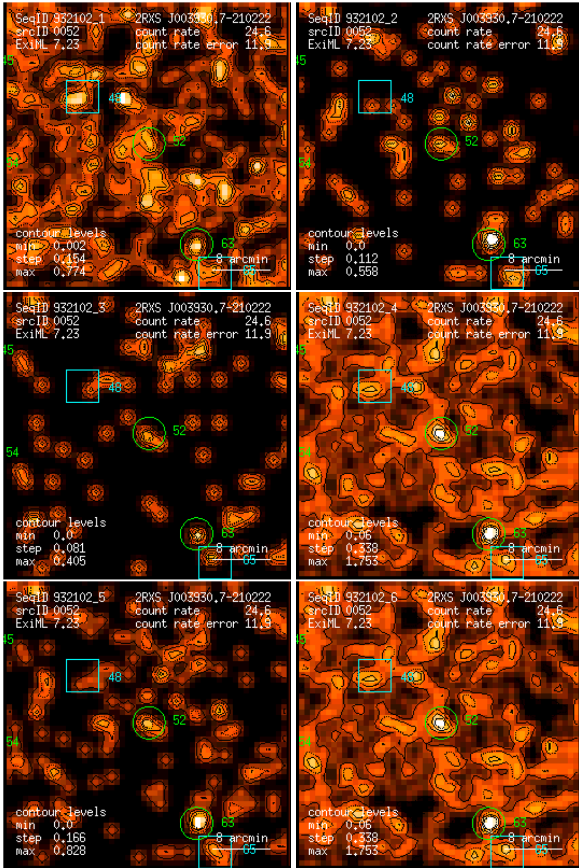
Figure 52: RASS 932102: detection 0052: band rate images, Gaussian filter: (1) PSPC channels 11 – 41, (2) 52 – 90, (3) 91 – 201, (4) 11 – 235, (5) 52 – 201, (6) 11 – 201. Broad band rates in counts/ks. Band rate contour levels in counts/ks/arcmin 2 .
