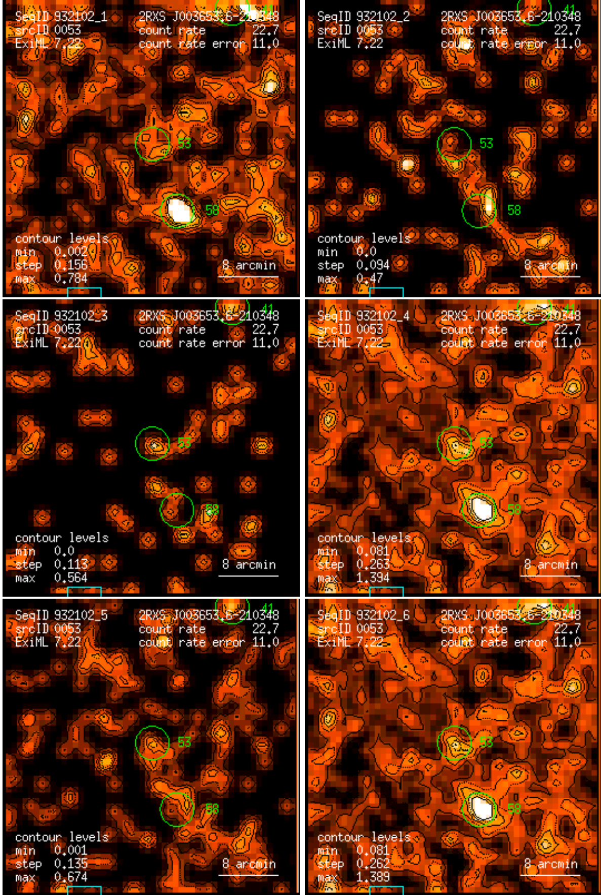
Figure 53: RASS 932102: detection 0053: band rate images, Gaussian filter: (1) PSPC channels 11 – 41, (2) 52 – 90, (3) 91 – 201, (4) 11 – 235, (5) 52 – 201, (6) 11 – 201. Broad band rates in counts/ks. Band rate contour levels in counts/ks/arcmin 2 .
