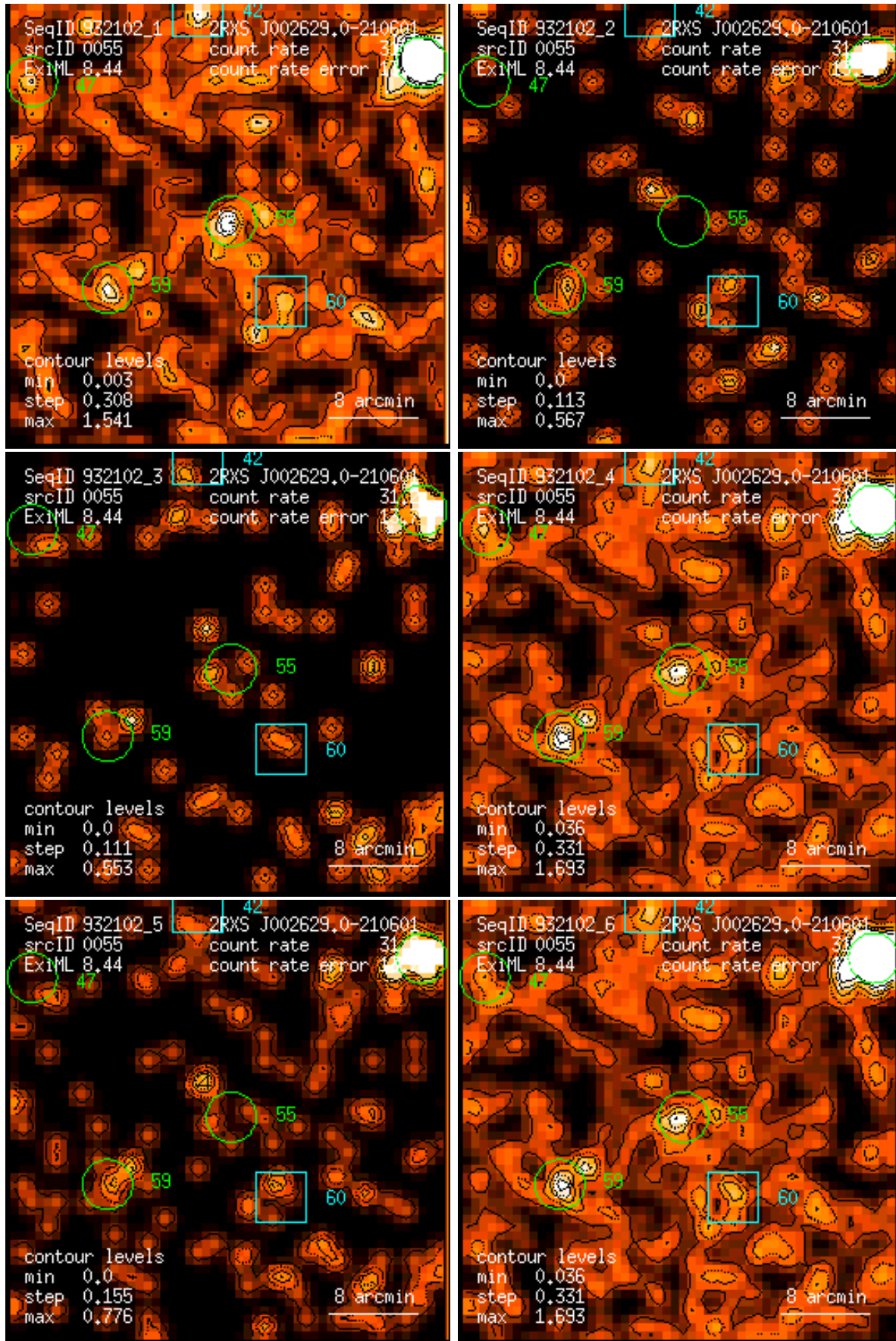
Figure 55: RASS 932102: detection 0055: band rate images, Gaussian filter: (1) PSPC channels 11 – 41, (2) 52 – 90, (3) 91 – 201, (4) 11 – 235, (5) 52 – 201, (6) 11 – 201. Broad band rates in counts/ks. Band rate contour levels in counts/ks/arcmin 2 .
