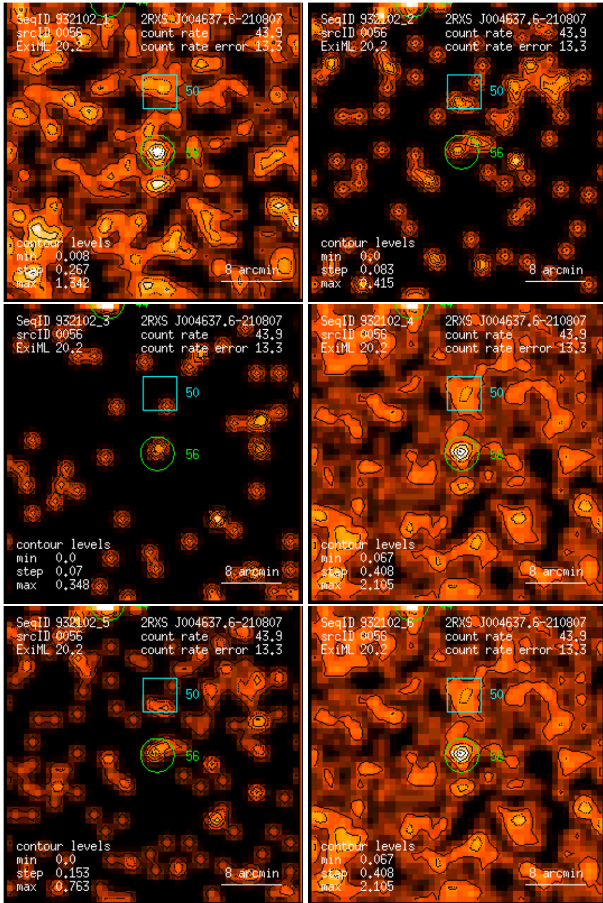
Figure 56: RASS 932102: detection 0056: band rate images, Gaussian filter: (1) PSPC channels 11 – 41, (2) 52 – 90, (3) 91 – 201, (4) 11 – 235, (5) 52 – 201, (6) 11 – 201. Broad band rates in counts/ks. Band rate contour levels in counts/ks/arcmin 2 .
