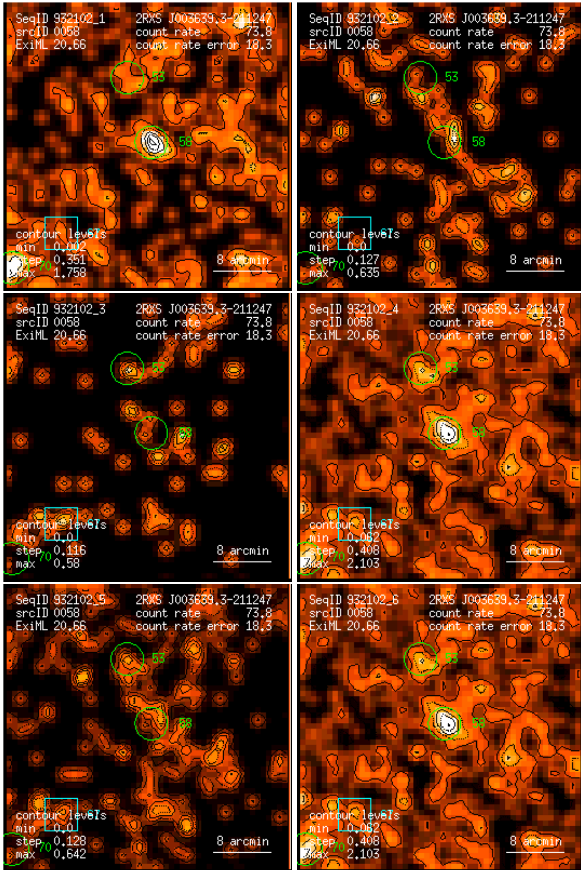
Figure 58: RASS 932102: detection 0058: band rate images, Gaussian filter: (1) PSPC channels 11 – 41, (2) 52 – 90, (3) 91 – 201, (4) 11 – 235, (5) 52 – 201, (6) 11 – 201. Broad band rates in counts/ks. Band rate contour levels in counts/ks/arcmin 2 .
