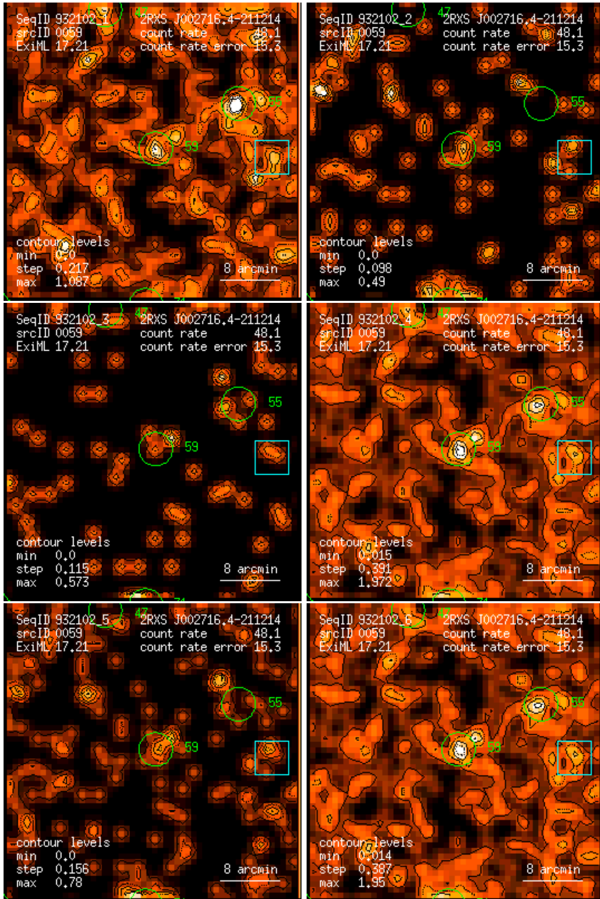
Figure 59: RASS 932102: detection 0059: band rate images, Gaussian filter: (1) PSPC channels 11 – 41, (2) 52 – 90, (3) 91 – 201, (4) 11 – 235, (5) 52 – 201, (6) 11 – 201. Broad band rates in counts/ks. Band rate contour levels in counts/ks/arcmin 2 .
