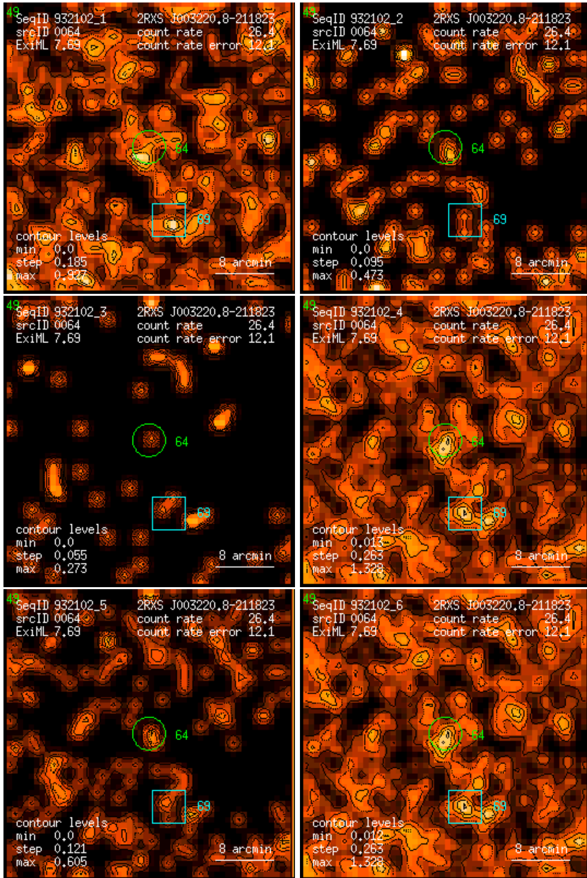
Figure 64: RASS 932102: detection 0064: band rate images, Gaussian filter: (1) PSPC channels 11 – 41, (2) 52 – 90, (3) 91 – 201, (4) 11 – 235, (5) 52 – 201, (6) 11 – 201. Broad band rates in counts/ks. Band rate contour levels in counts/ks/arcmin 2 .
