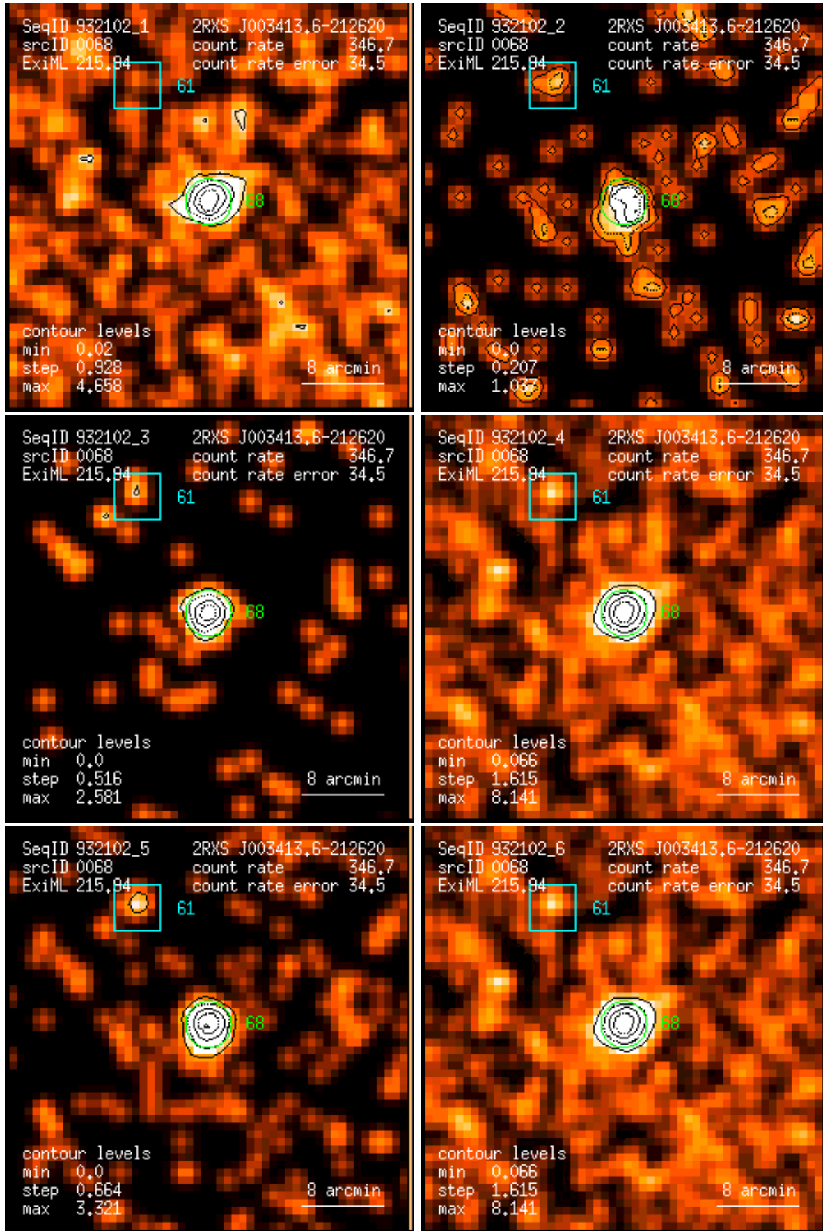
Figure 68: RASS 932102: detection 0068: band rate images, Gaussian filter: (1) PSPC channels 11 – 41, (2) 52 – 90, (3) 91 – 201, (4) 11 – 235, (5) 52 – 201, (6) 11 – 201. Broad band rates in counts/ks. Band rate contour levels in counts/ks/arcmin 2 .
