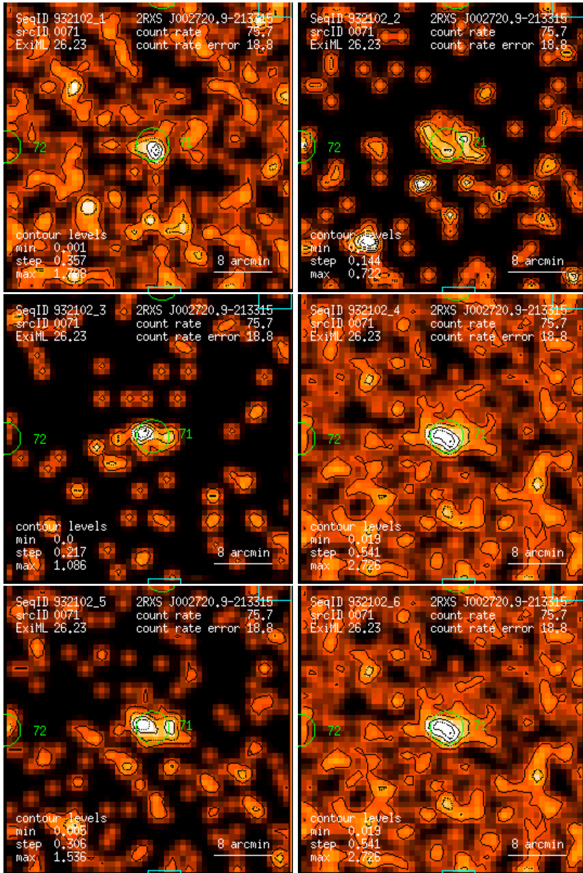
Figure 71: RASS 932102: detection 0071: band rate images, Gaussian filter: (1) PSPC channels 11 – 41, (2) 52 – 90, (3) 91 – 201, (4) 11 – 235, (5) 52 – 201, (6) 11 – 201. Broad band rates in counts/ks. Band rate contour levels in counts/ks/arcmin 2 .
