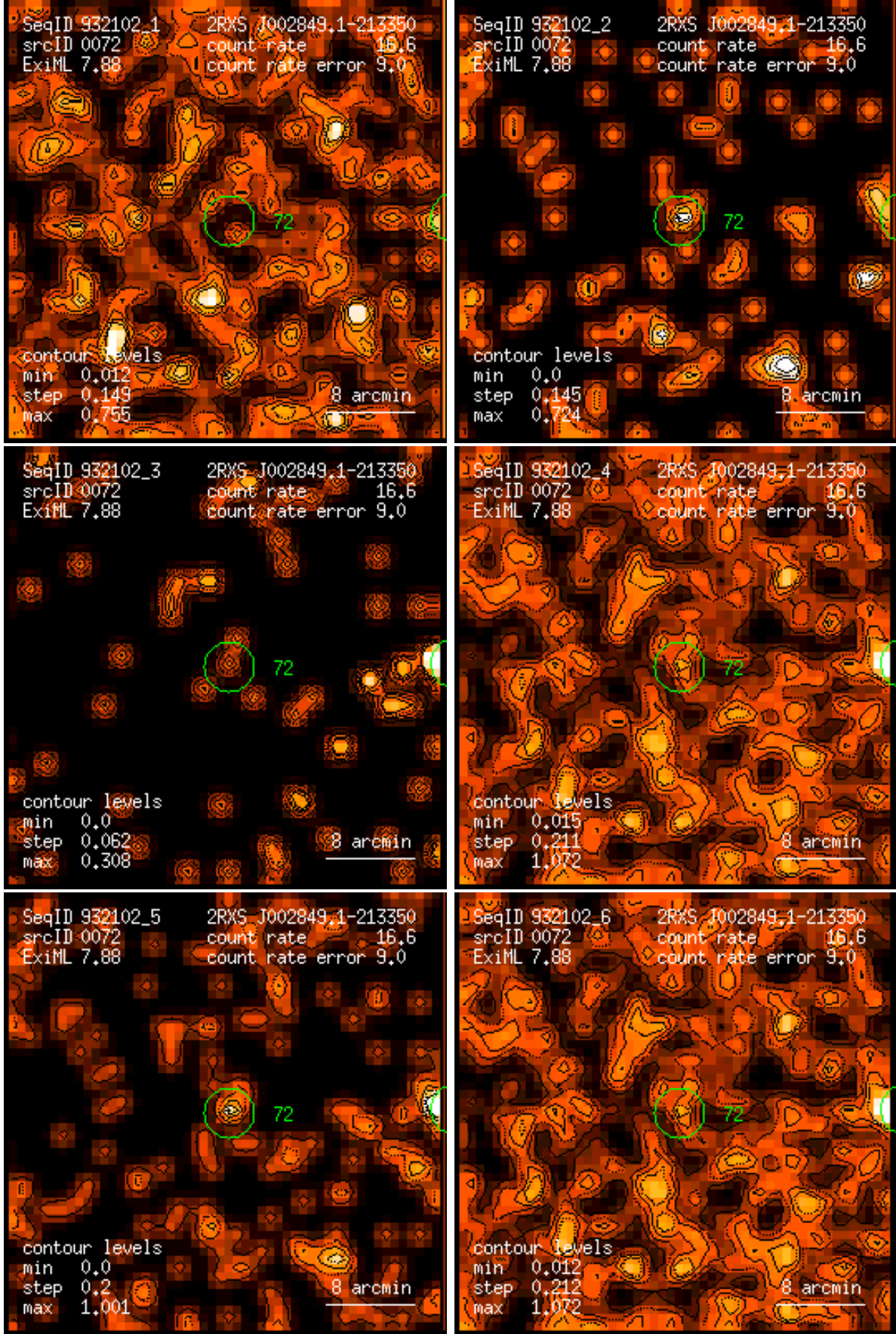
Figure 72: RASS 932102: detection 0072: band rate images, Gaussian filter: (1) PSPC channels 11 – 41, (2) 52 – 90, (3) 91 – 201, (4) 11 – 235, (5) 52 – 201, (6) 11 – 201. Broad band rates in counts/ks. Band rate contour levels in counts/ks/arcmin 2 .
