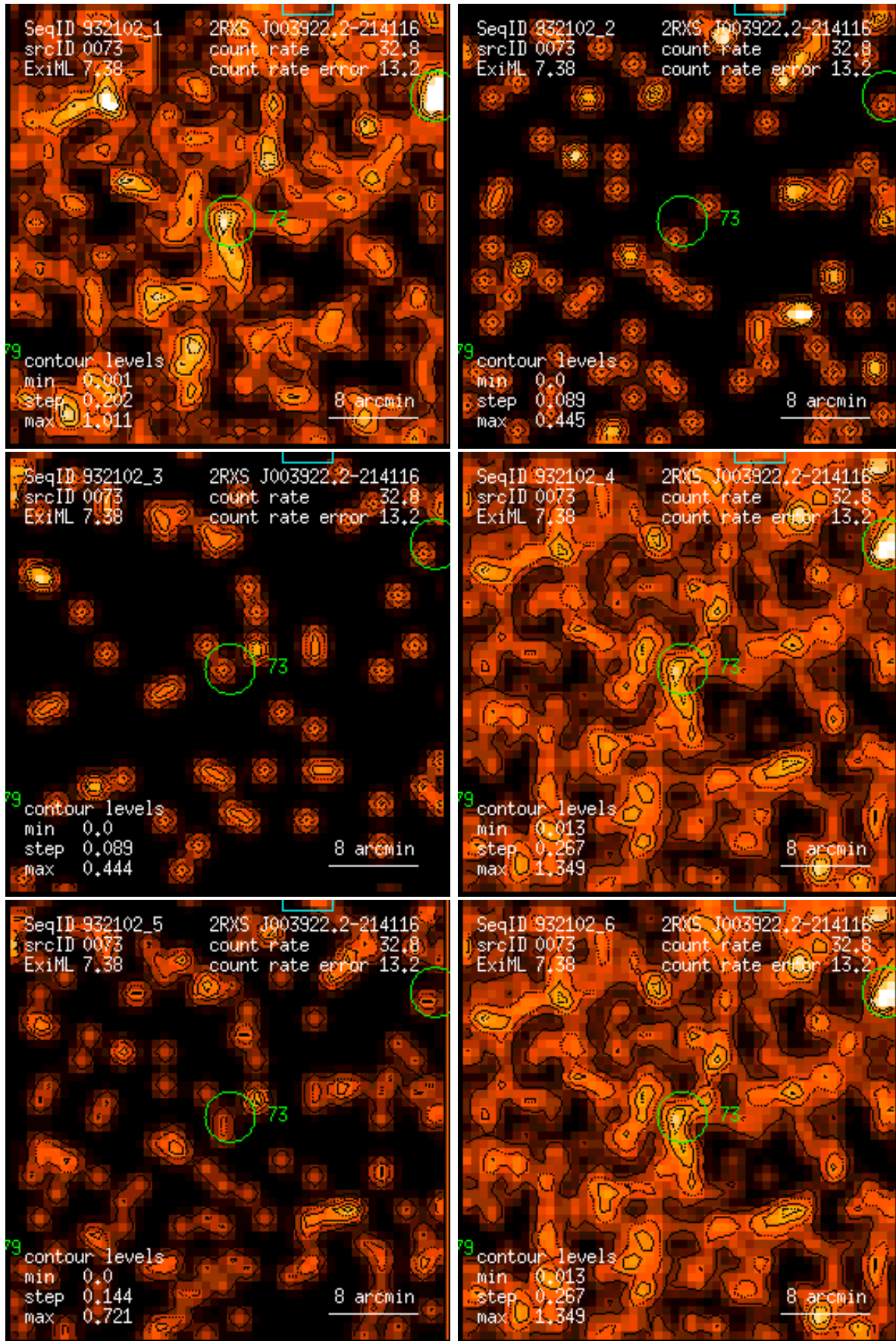
Figure 73: RASS 932102: detection 0073: band rate images, Gaussian filter: (1) PSPC channels 11 – 41, (2) 52 – 90, (3) 91 – 201, (4) 11 – 235, (5) 52 – 201, (6) 11 – 201. Broad band rates in counts/ks. Band rate contour levels in counts/ks/arcmin 2 .
