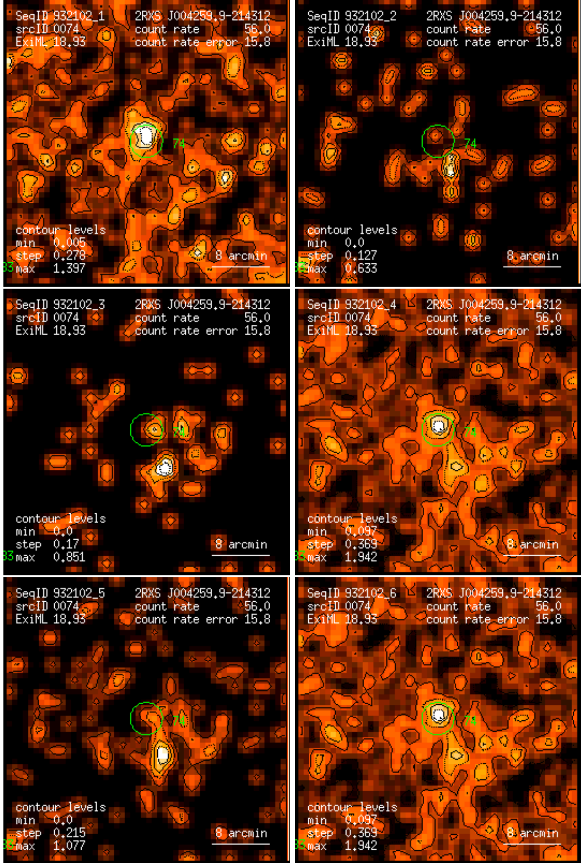
Figure 74: RASS 932102: detection 0074: band rate images, Gaussian filter: (1) PSPC channels 11 – 41, (2) 52 – 90, (3) 91 – 201, (4) 11 – 235, (5) 52 – 201, (6) 11 – 201. Broad band rates in counts/ks. Band rate contour levels in counts/ks/arcmin 2 .
