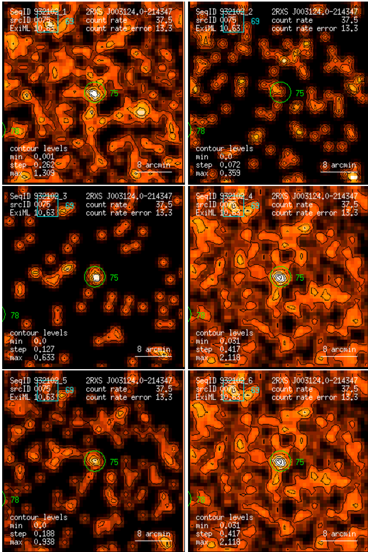
Figure 75: RASS 932102: detection 0075: band rate images, Gaussian filter: (1) PSPC channels 11 – 41, (2) 52 – 90, (3) 91 – 201, (4) 11 – 235, (5) 52 – 201, (6) 11 – 201. Broad band rates in counts/ks. Band rate contour levels in counts/ks/arcmin 2 .
