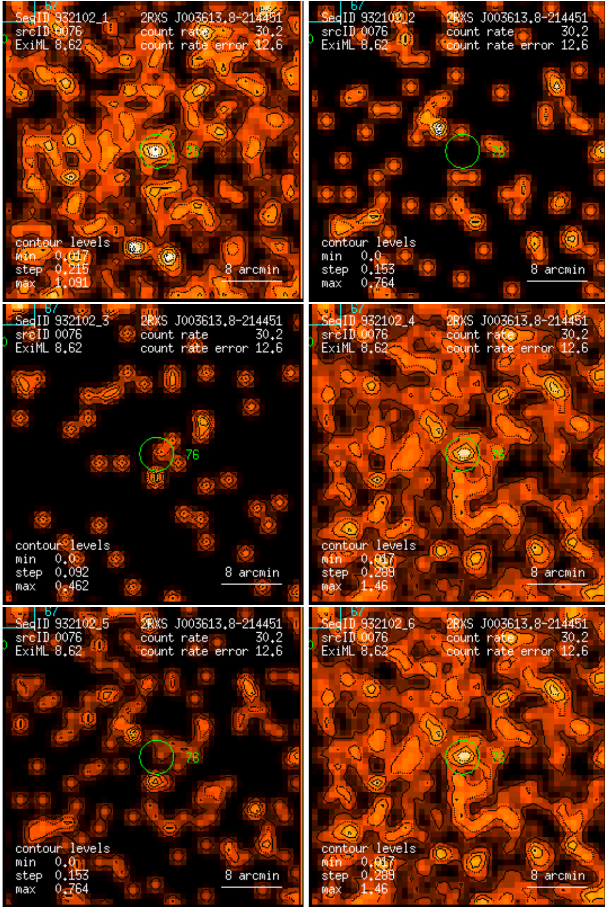
Figure 76: RASS 932102: detection 0076: band rate images, Gaussian filter: (1) PSPC channels 11 – 41, (2) 52 – 90, (3) 91 – 201, (4) 11 – 235, (5) 52 – 201, (6) 11 – 201. Broad band rates in counts/ks. Band rate contour levels in counts/ks/arcmin 2 .
