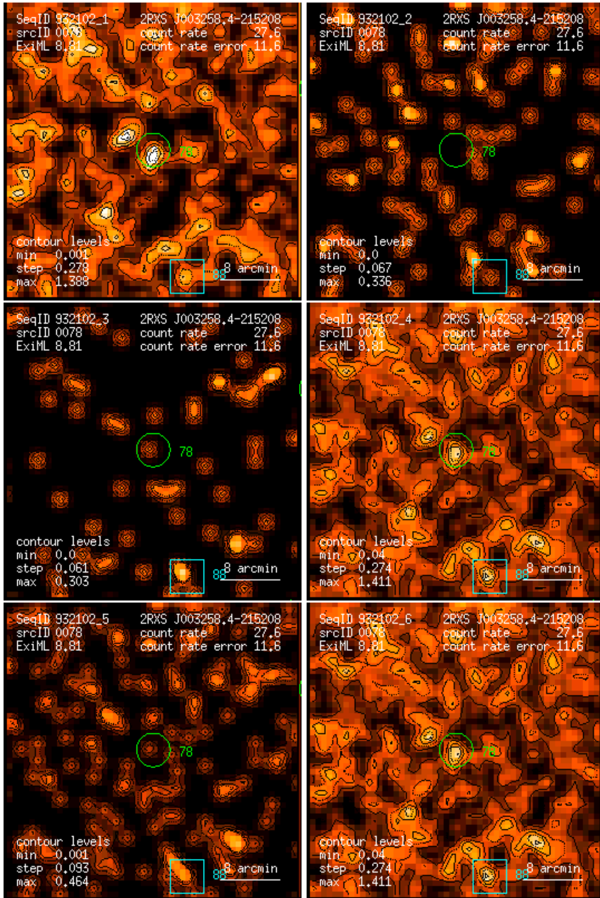
Figure 78: RASS 932102: detection 0078: band rate images, Gaussian filter: (1) PSPC channels 11 – 41, (2) 52 – 90, (3) 91 – 201, (4) 11 – 235, (5) 52 – 201, (6) 11 – 201. Broad band rates in counts/ks. Band rate contour levels in counts/ks/arcmin 2 .
