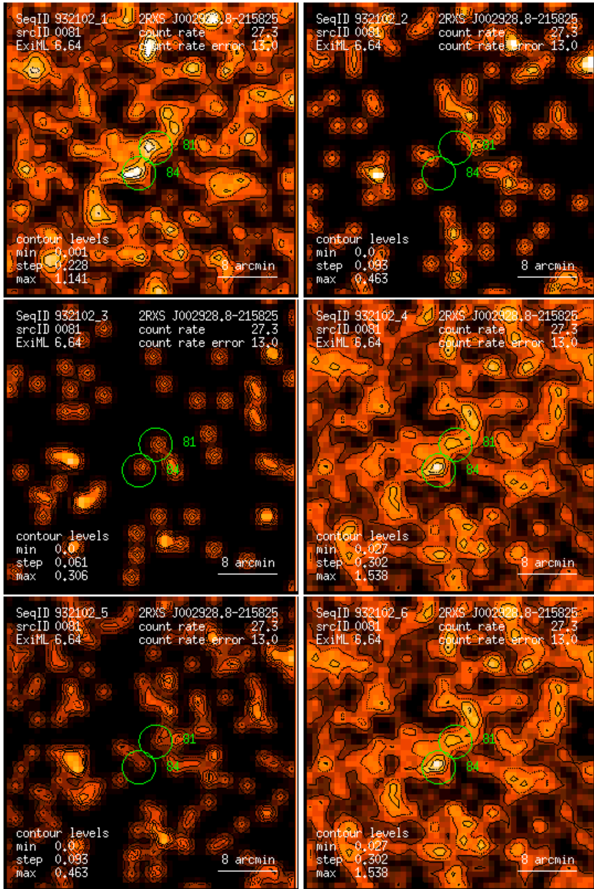
Figure 81: RASS 932102: detection 0081: band rate images, Gaussian filter: (1) PSPC channels 11 – 41, (2) 52 – 90, (3) 91 – 201, (4) 11 – 235, (5) 52 – 201, (6) 11 – 201. Broad band rates in counts/ks. Band rate contour levels in counts/ks/arcmin 2 .
