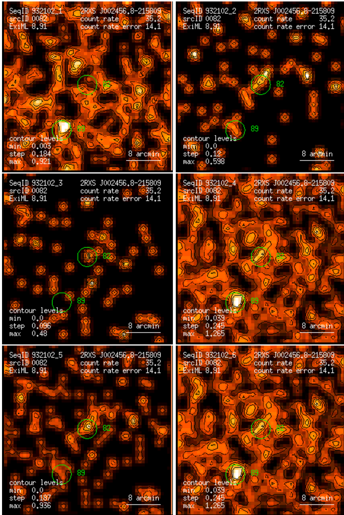
Figure 82: RASS 932102: detection 0082: band rate images, Gaussian filter: (1) PSPC channels 11 – 41, (2) 52 – 90, (3) 91 – 201, (4) 11 – 235, (5) 52 – 201, (6) 11 – 201. Broad band rates in counts/ks. Band rate contour levels in counts/ks/arcmin 2 .
