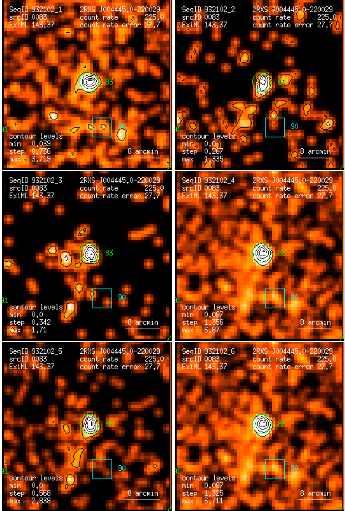
Figure 83: RASS 932102: detection 0083: band rate images, Gaussian filter: (1) PSPC channels 11 – 41, (2) 52 – 90, (3) 91 – 201, (4) 11 – 235, (5) 52 – 201, (6) 11 – 201. Broad band rates in counts/ks. Band rate contour levels in counts/ks/arcmin 2 .
