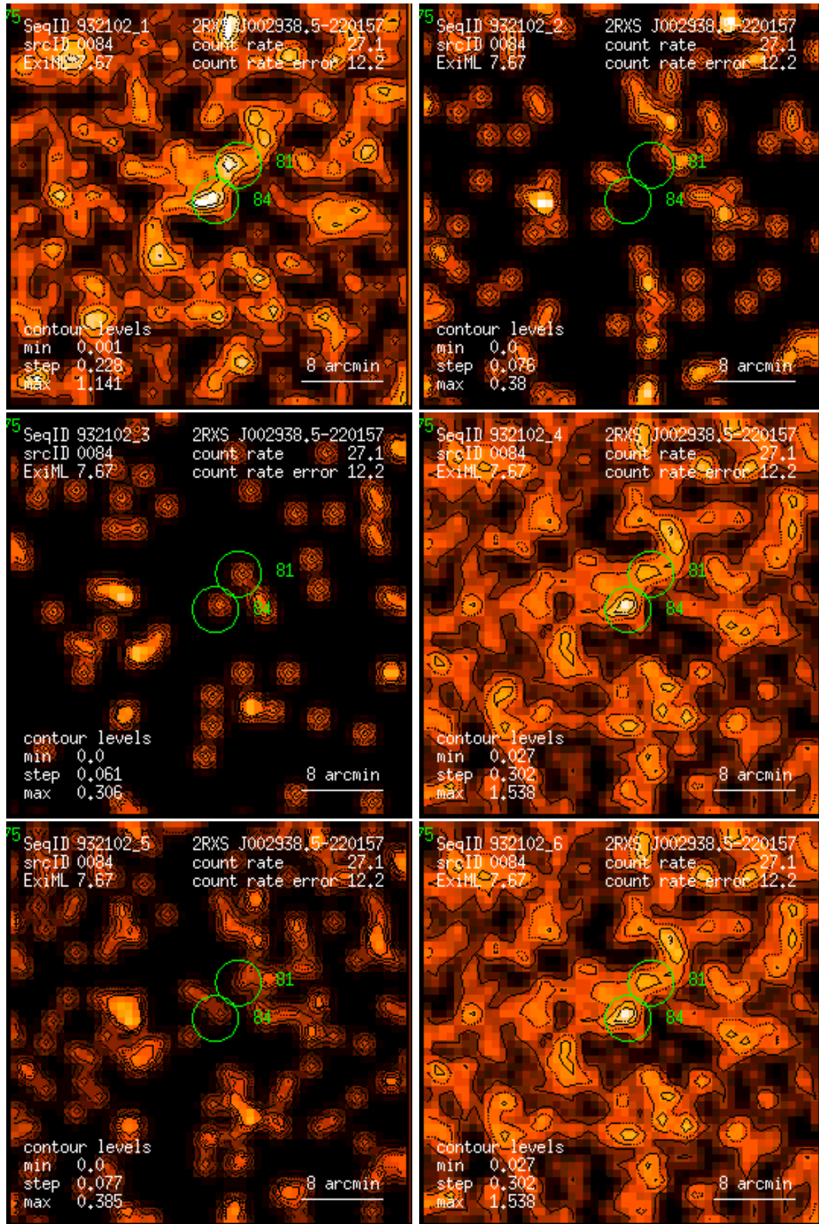
Figure 84: RASS 932102: detection 0084: band rate images, Gaussian filter: (1) PSPC channels 11 – 41, (2) 52 – 90, (3) 91 – 201, (4) 11 – 235, (5) 52 – 201, (6) 11 – 201. Broad band rates in counts/ks. Band rate contour levels in counts/ks/arcmin 2 .
