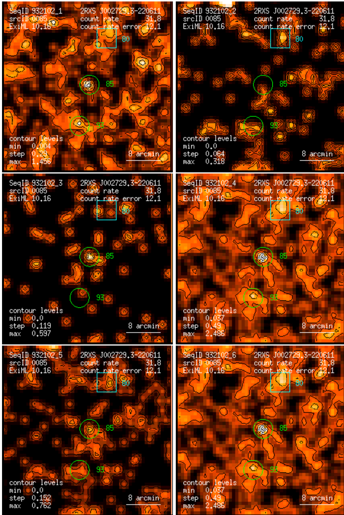
Figure 85: RASS 932102: detection 0085: band rate images, Gaussian filter: (1) PSPC channels 11 – 41, (2) 52 – 90, (3) 91 – 201, (4) 11 – 235, (5) 52 – 201, (6) 11 – 201. Broad band rates in counts/ks. Band rate contour levels in counts/ks/arcmin 2 .
