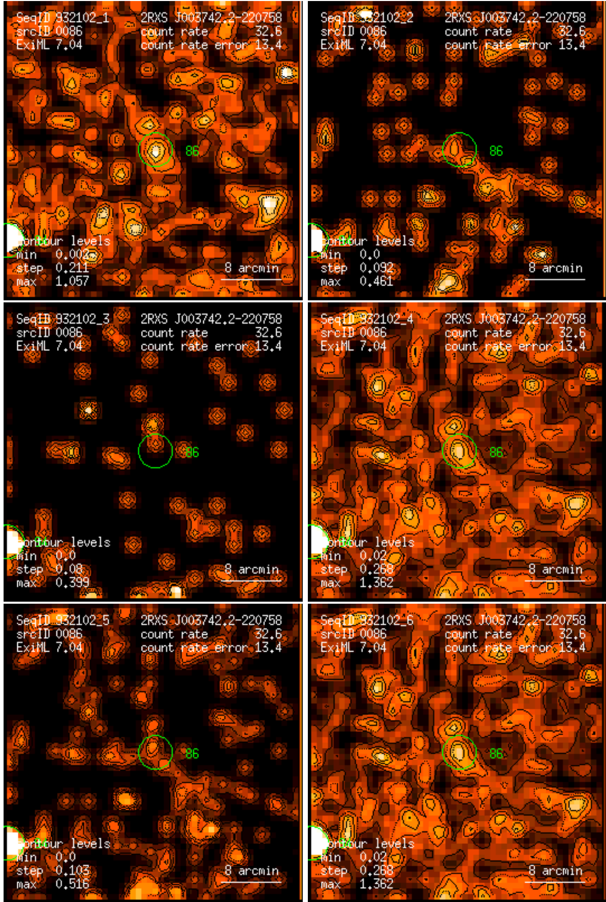
Figure 86: RASS 932102: detection 0086: band rate images, Gaussian filter: (1) PSPC channels 11 – 41, (2) 52 – 90, (3) 91 – 201, (4) 11 – 235, (5) 52 – 201, (6) 11 – 201. Broad band rates in counts/ks. Band rate contour levels in counts/ks/arcmin 2 .
