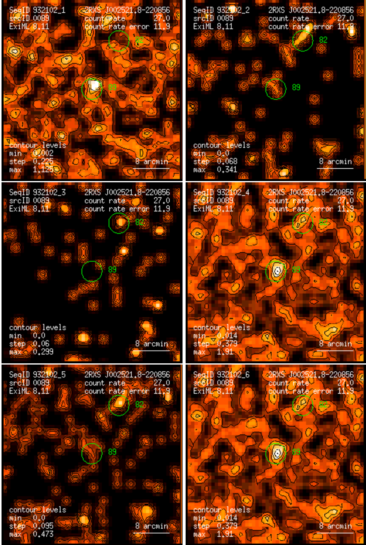
Figure 89: RASS 932102: detection 0089: band rate images, Gaussian filter: (1) PSPC channels 11 – 41, (2) 52 – 90, (3) 91 – 201, (4) 11 – 235, (5) 52 – 201, (6) 11 – 201. Broad band rates in counts/ks. Band rate contour levels in counts/ks/arcmin 2 .
