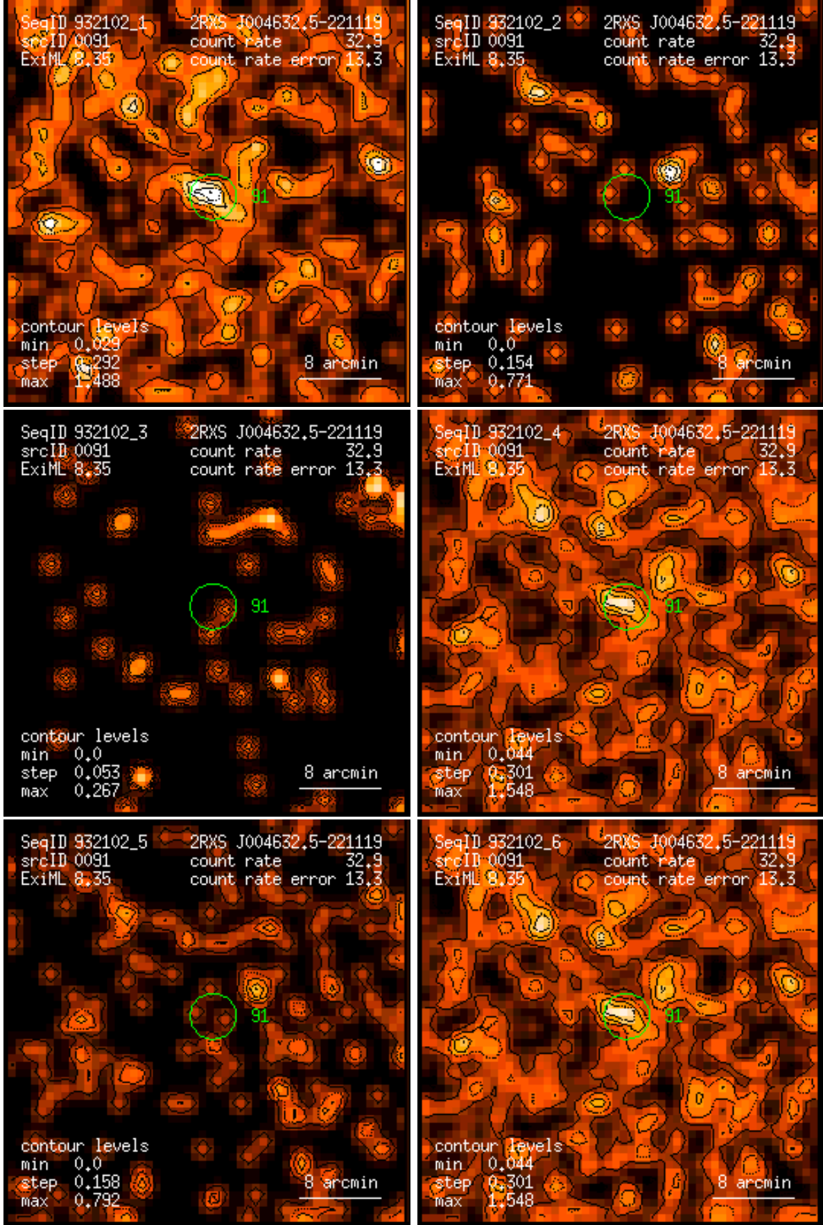
Figure 91: RASS 932102: detection 0091: band rate images, Gaussian filter: (1) PSPC channels 11 – 41, (2) 52 – 90, (3) 91 – 201, (4) 11 – 235, (5) 52 – 201, (6) 11 – 201. Broad band rates in counts/ks. Band rate contour levels in counts/ks/arcmin 2 .
