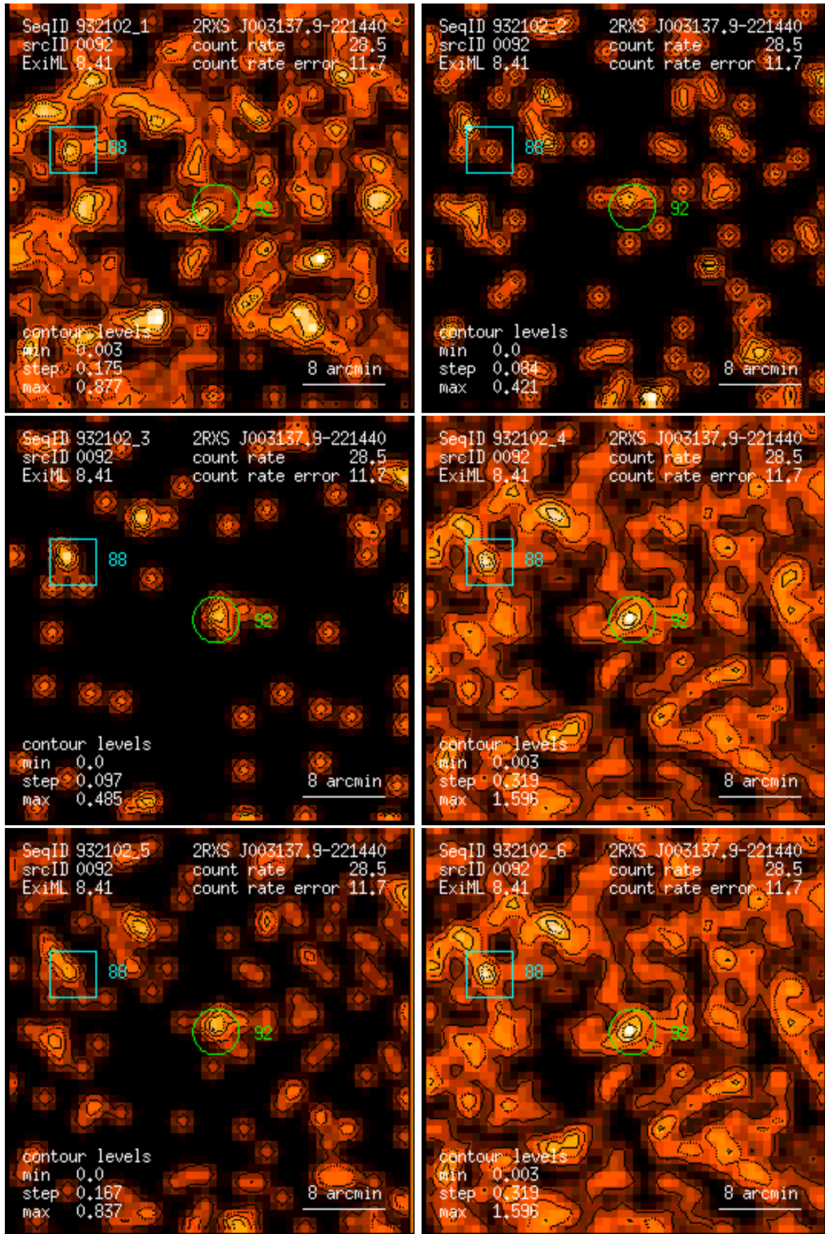
Figure 92: RASS 932102: detection 0092: band rate images, Gaussian filter: (1) PSPC channels 11 – 41, (2) 52 – 90, (3) 91 – 201, (4) 11 – 235, (5) 52 – 201, (6) 11 – 201. Broad band rates in counts/ks. Band rate contour levels in counts/ks/arcmin 2 .
