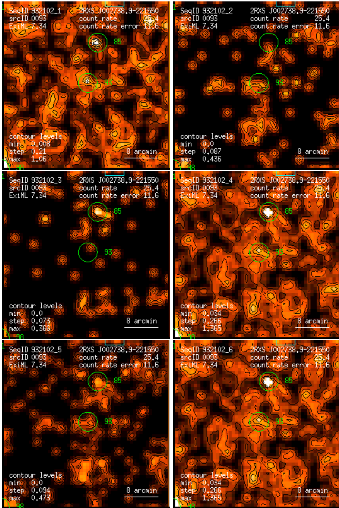
Figure 93: RASS 932102: detection 0093: band rate images, Gaussian filter: (1) PSPC channels 11 – 41, (2) 52 – 90, (3) 91 – 201, (4) 11 – 235, (5) 52 – 201, (6) 11 – 201. Broad band rates in counts/ks. Band rate contour levels in counts/ks/arcmin 2 .
