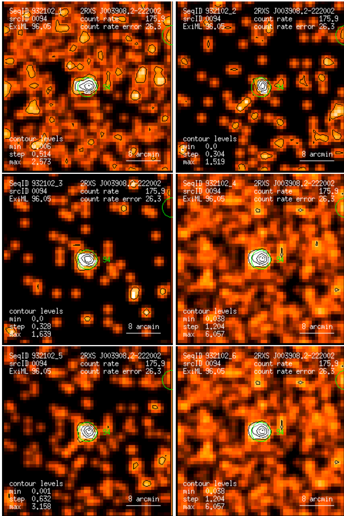
Figure 94: RASS 932102: detection 0094: band rate images, Gaussian filter: (1) PSPC channels 11 – 41, (2) 52 – 90, (3) 91 – 201, (4) 11 – 235, (5) 52 – 201, (6) 11 – 201. Broad band rates in counts/ks. Band rate contour levels in counts/ks/arcmin 2 .
