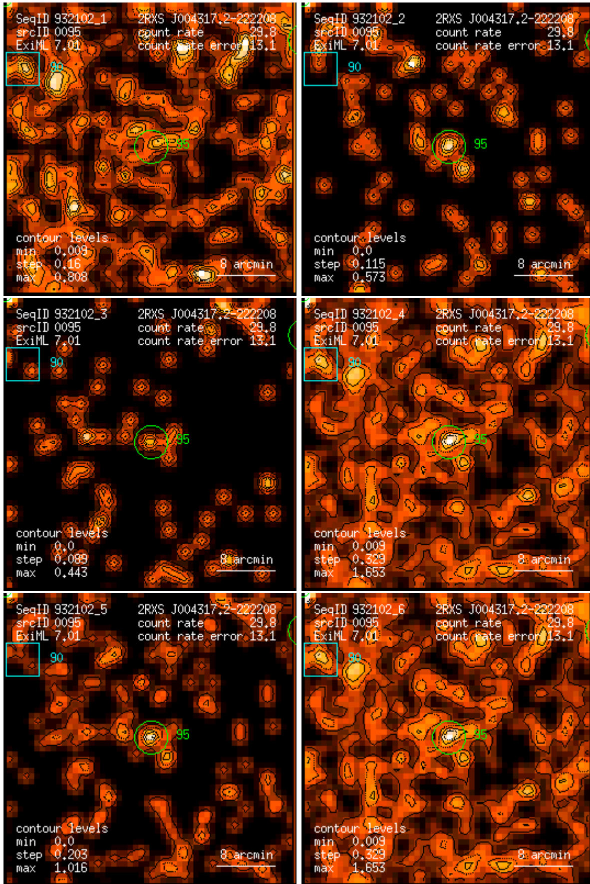
Figure 95: RASS 932102: detection 0095: band rate images, Gaussian filter: (1) PSPC channels 11 – 41, (2) 52 – 90, (3) 91 – 201, (4) 11 – 235, (5) 52 – 201, (6) 11 – 201. Broad band rates in counts/ks. Band rate contour levels in counts/ks/arcmin 2 .
