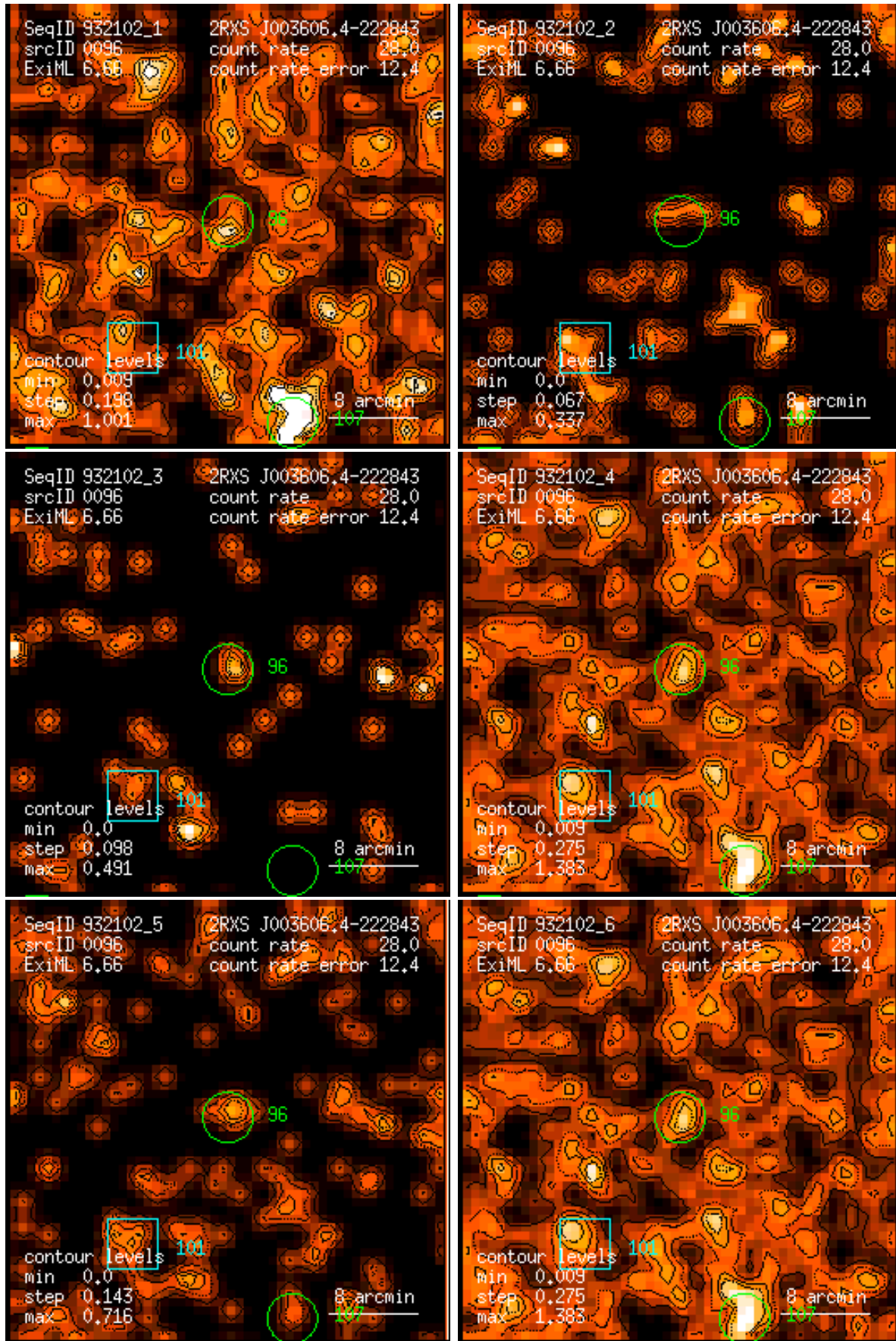
Figure 96: RASS 932102: detection 0096: band rate images, Gaussian filter: (1) PSPC channels 11 – 41, (2) 52 – 90, (3) 91 – 201, (4) 11 – 235, (5) 52 – 201, (6) 11 – 201. Broad band rates in counts/ks. Band rate contour levels in counts/ks/arcmin 2 .
