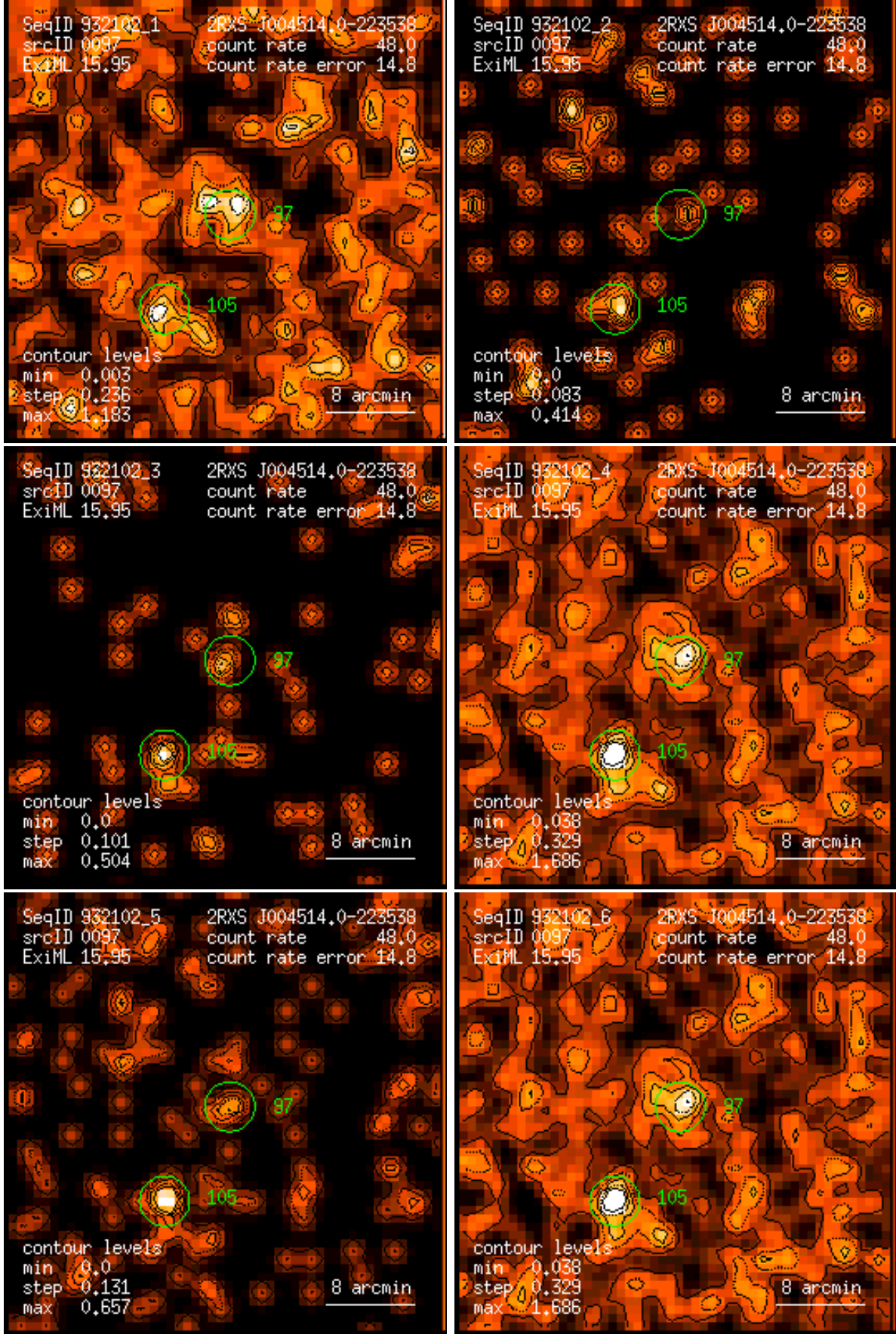
Figure 97: RASS 932102: detection 0097: band rate images, Gaussian filter: (1) PSPC channels 11 – 41, (2) 52 – 90, (3) 91 – 201, (4) 11 – 235, (5) 52 – 201, (6) 11 – 201. Broad band rates in counts/ks. Band rate contour levels in counts/ks/arcmin 2 .
