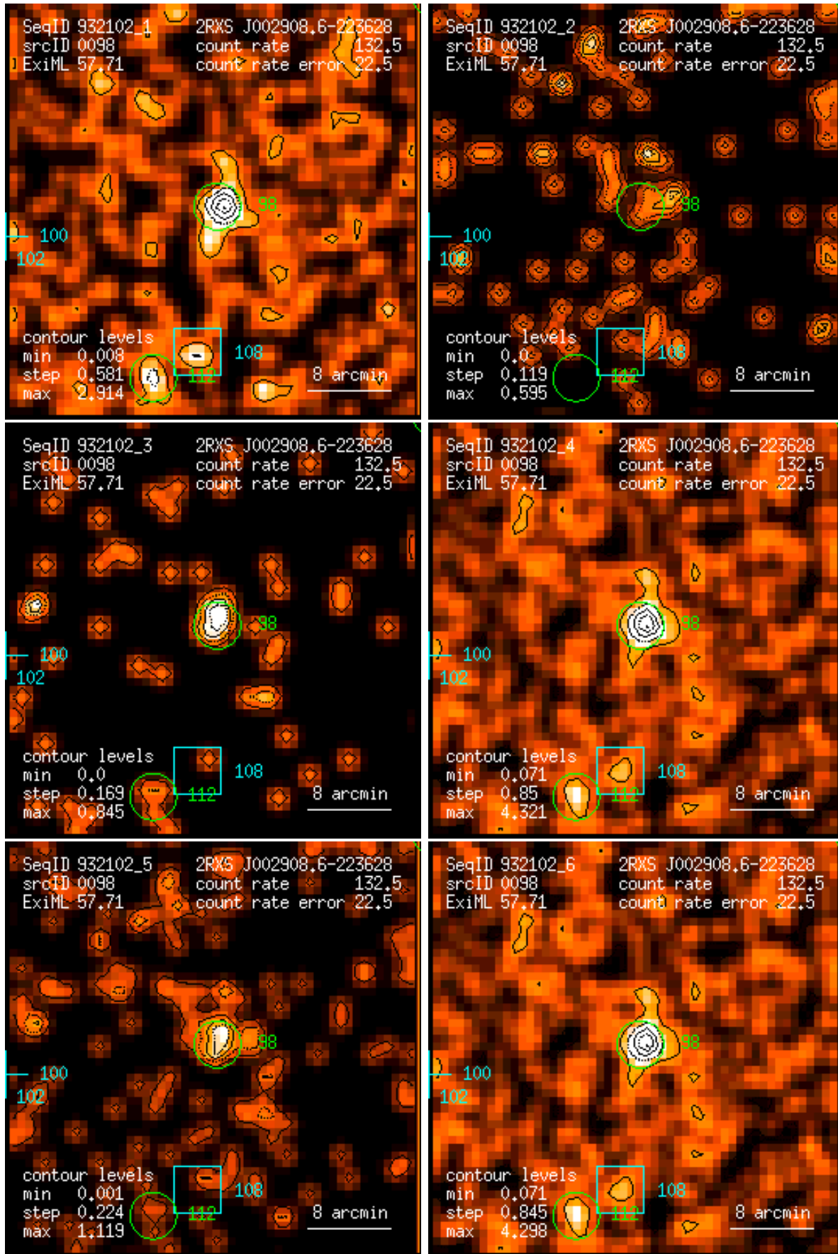
Figure 98: RASS 932102: detection 0098: band rate images, Gaussian filter: (1) PSPC channels 11 – 41, (2) 52 – 90, (3) 91 – 201, (4) 11 – 235, (5) 52 – 201, (6) 11 – 201. Broad band rates in counts/ks. Band rate contour levels in counts/ks/arcmin 2 .
