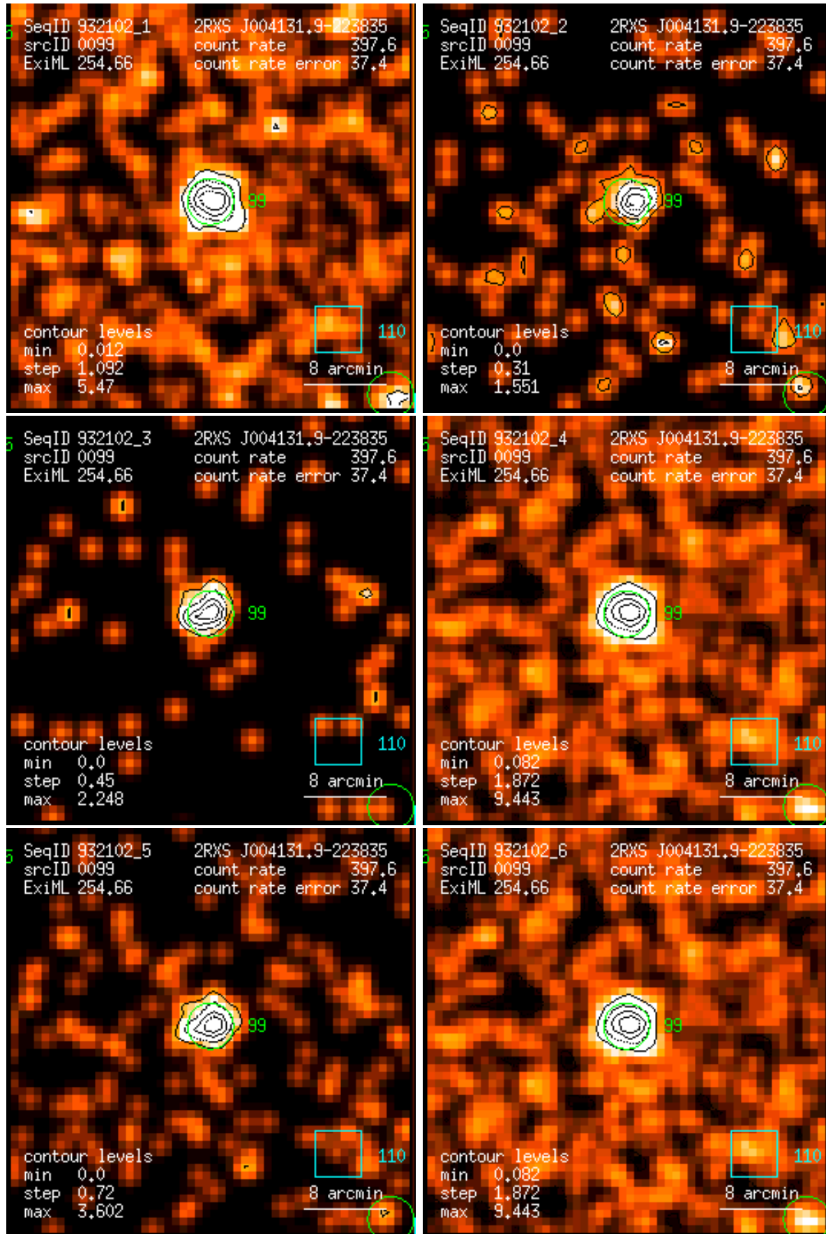
Figure 99: RASS 932102: detection 0099: band rate images, Gaussian filter: (1) PSPC channels 11 – 41, (2) 52 – 90, (3) 91 – 201, (4) 11 – 235, (5) 52 – 201, (6) 11 – 201. Broad band rates in counts/ks. Band rate contour levels in counts/ks/arcmin 2 .
