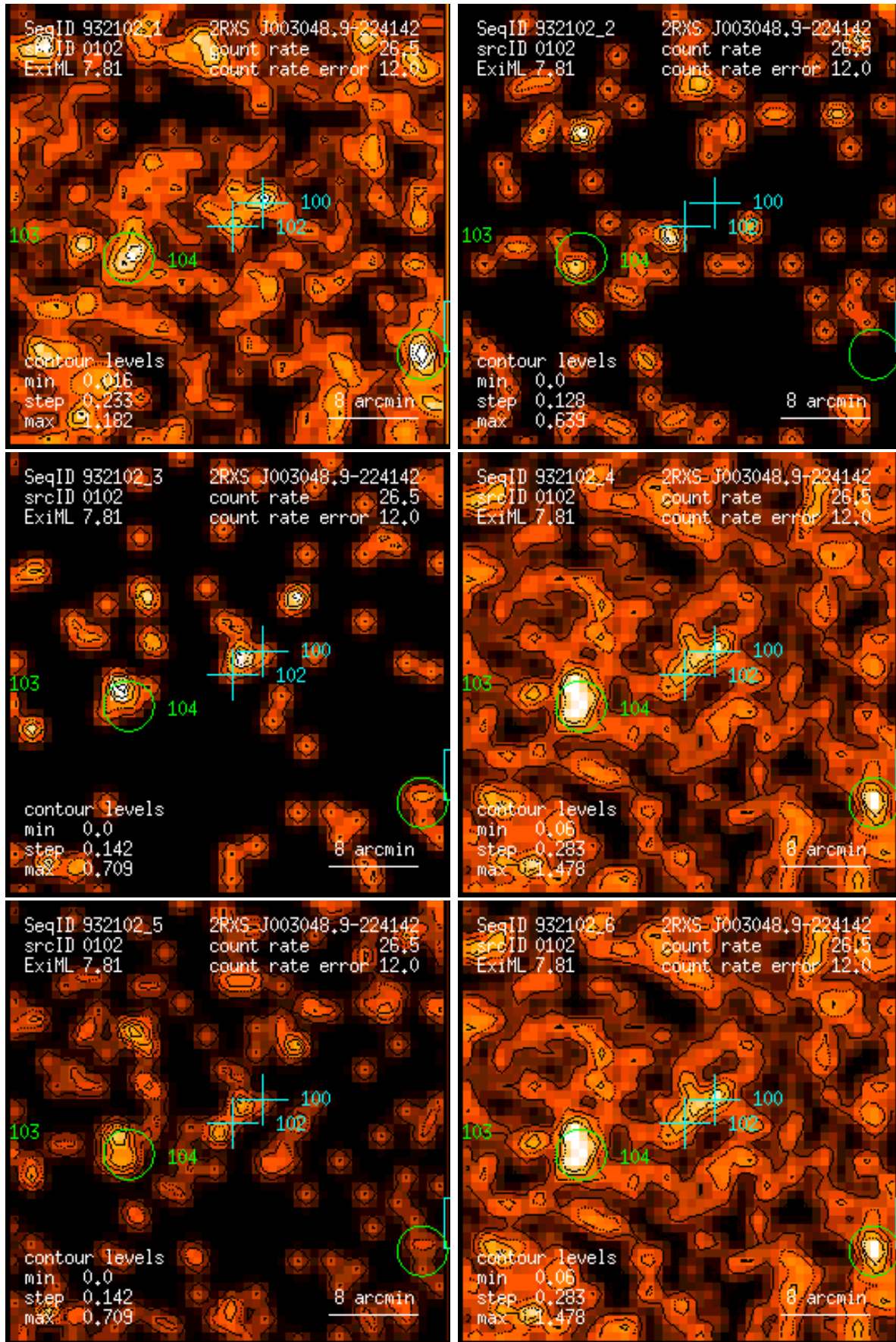
Figure 102: RASS 932102: detection 0102: band rate images, Gaussian filter: (1) PSPC channels 11 – 41, (2) 52 – 90, (3) 91 – 201, (4) 11 – 235, (5) 52 – 201, (6) 11 – 201. Broad band rates in counts/ks. Band rate contour levels in counts/ks/arcmin 2 .
