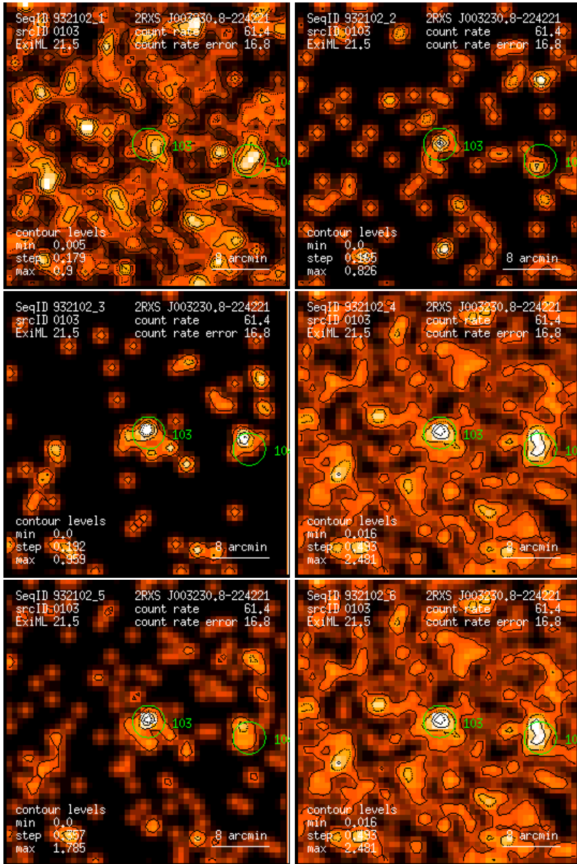
Figure 103: RASS 932102: detection 0103: band rate images, Gaussian filter: (1) PSPC channels 11 – 41, (2) 52 – 90, (3) 91 – 201, (4) 11 – 235, (5) 52 – 201, (6) 11 – 201. Broad band rates in counts/ks. Band rate contour levels in counts/ks/arcmin 2 .
