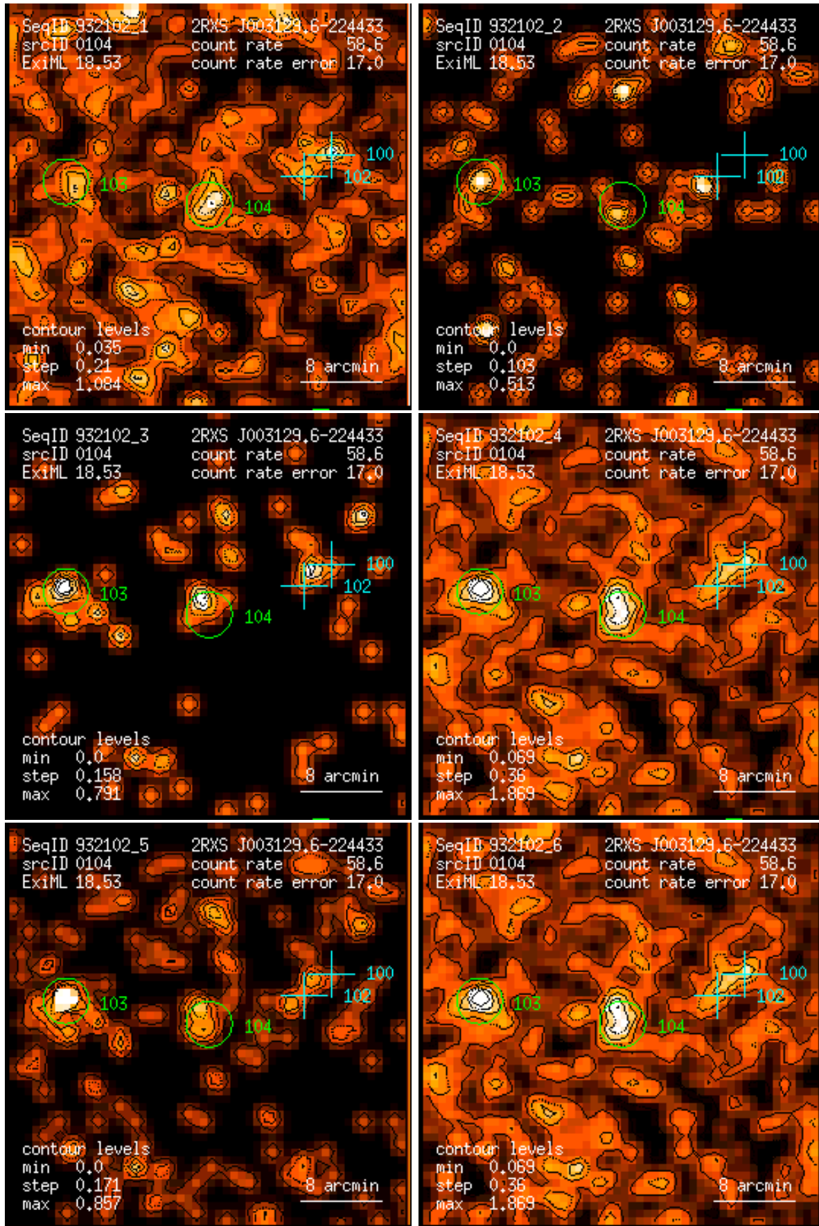
Figure 104: RASS 932102: detection 0104: band rate images, Gaussian filter: (1) PSPC channels 11 – 41, (2) 52 – 90, (3) 91 – 201, (4) 11 – 235, (5) 52 – 201, (6) 11 – 201. Broad band rates in counts/ks. Band rate contour levels in counts/ks/arcmin 2 .
