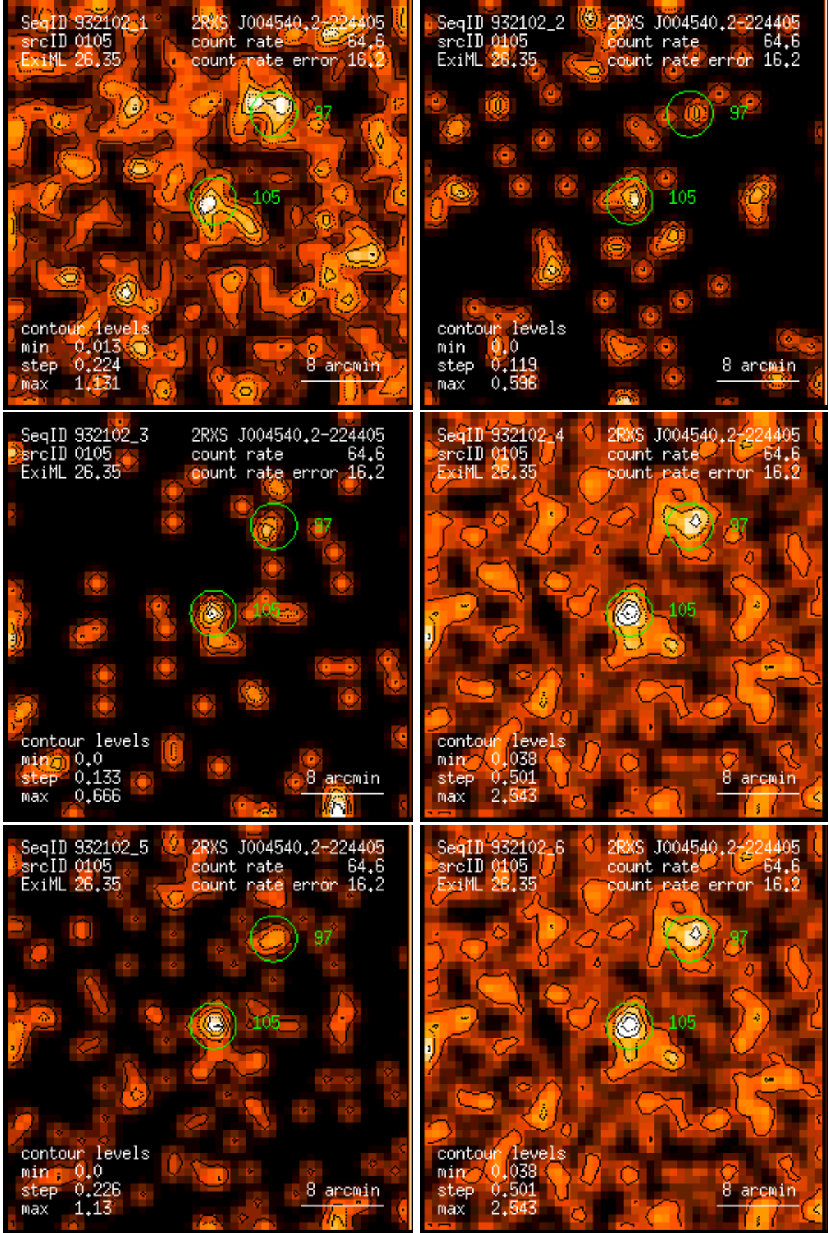
Figure 105: RASS 932102: detection 0105: band rate images, Gaussian filter: (1) PSPC channels 11 – 41, (2) 52 – 90, (3) 91 – 201, (4) 11 – 235, (5) 52 – 201, (6) 11 – 201. Broad band rates in counts/ks. Band rate contour levels in counts/ks/arcmin 2 .
