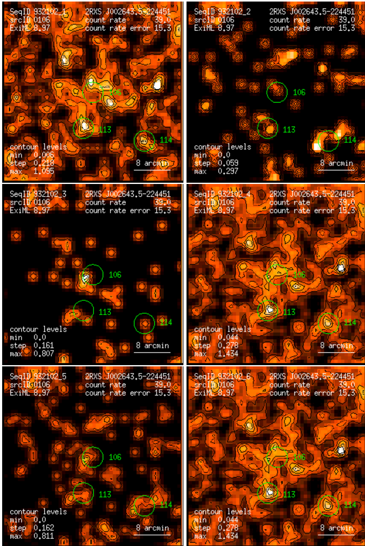
Figure 106: RASS 932102: detection 0106: band rate images, Gaussian filter: (1) PSPC channels 11 – 41, (2) 52 – 90, (3) 91 – 201, (4) 11 – 235, (5) 52 – 201, (6) 11 – 201. Broad band rates in counts/ks. Band rate contour levels in counts/ks/arcmin 2 .
