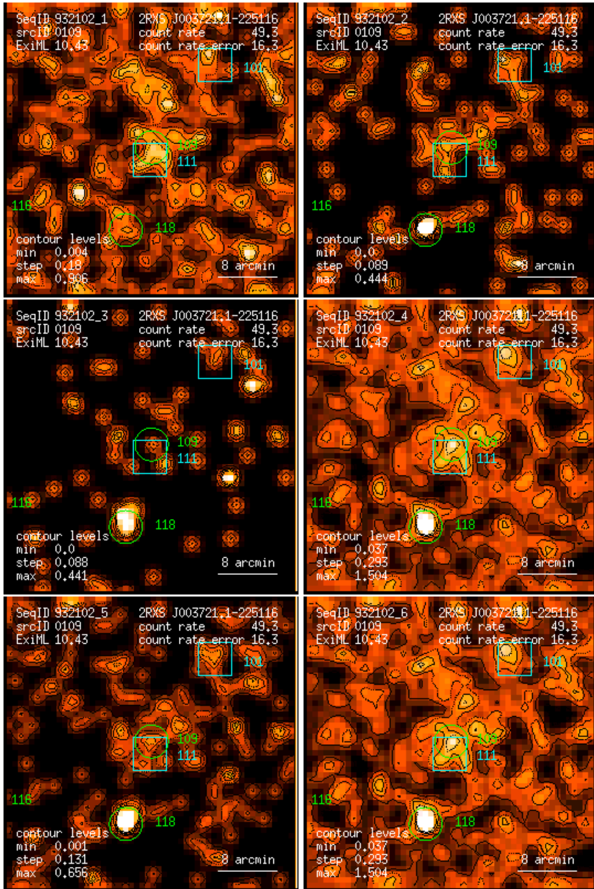
Figure 109: RASS 932102: detection 0109: band rate images, Gaussian filter: (1) PSPC channels 11 – 41, (2) 52 – 90, (3) 91 – 201, (4) 11 – 235, (5) 52 – 201, (6) 11 – 201. Broad band rates in counts/ks. Band rate contour levels in counts/ks/arcmin 2 .
