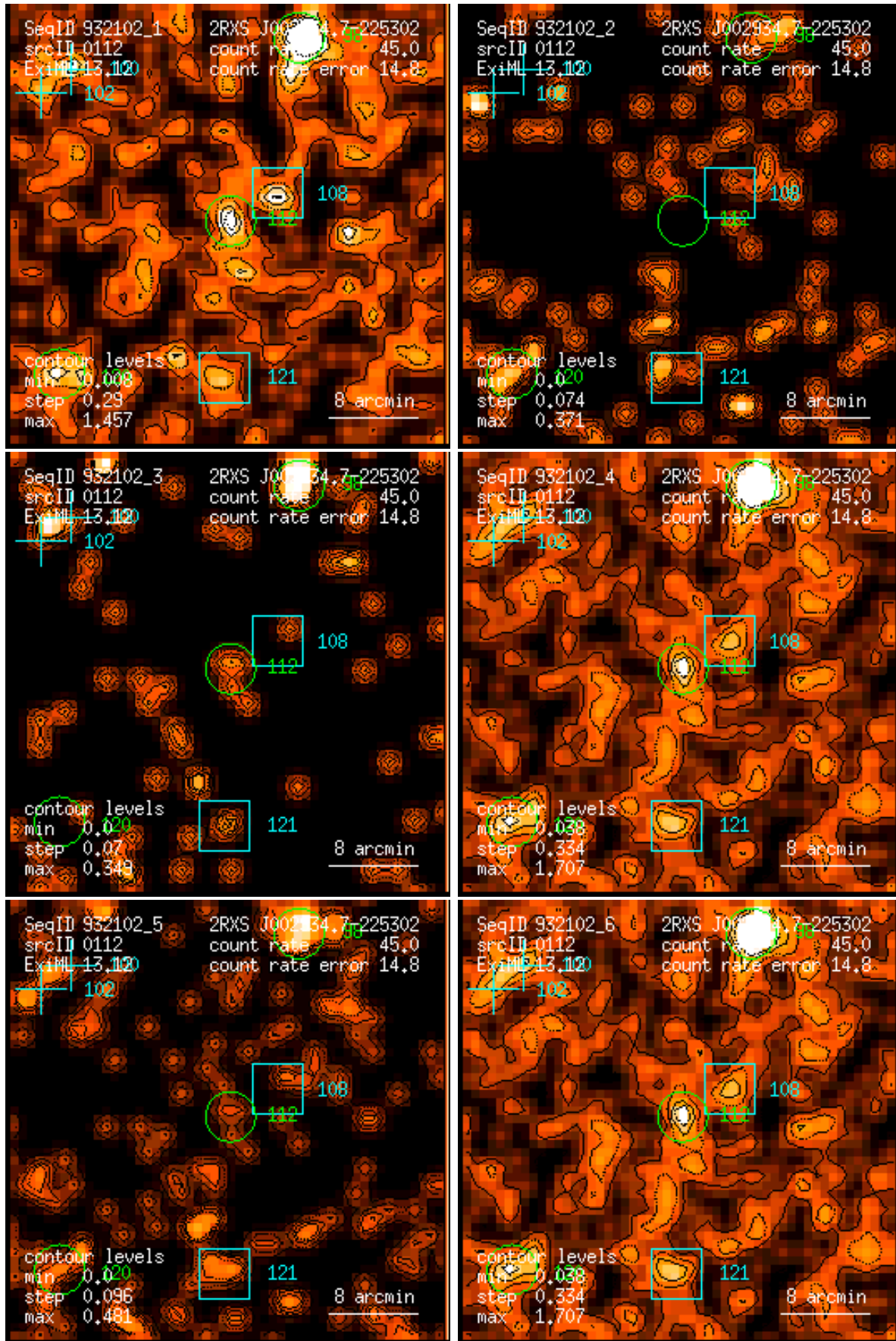
Figure 112: RASS 932102: detection 0112: band rate images, Gaussian filter: (1) PSPC channels 11 – 41, (2) 52 – 90, (3) 91 – 201, (4) 11 – 235, (5) 52 – 201, (6) 11 – 201. Broad band rates in counts/ks. Band rate contour levels in counts/ks/arcmin 2 .
