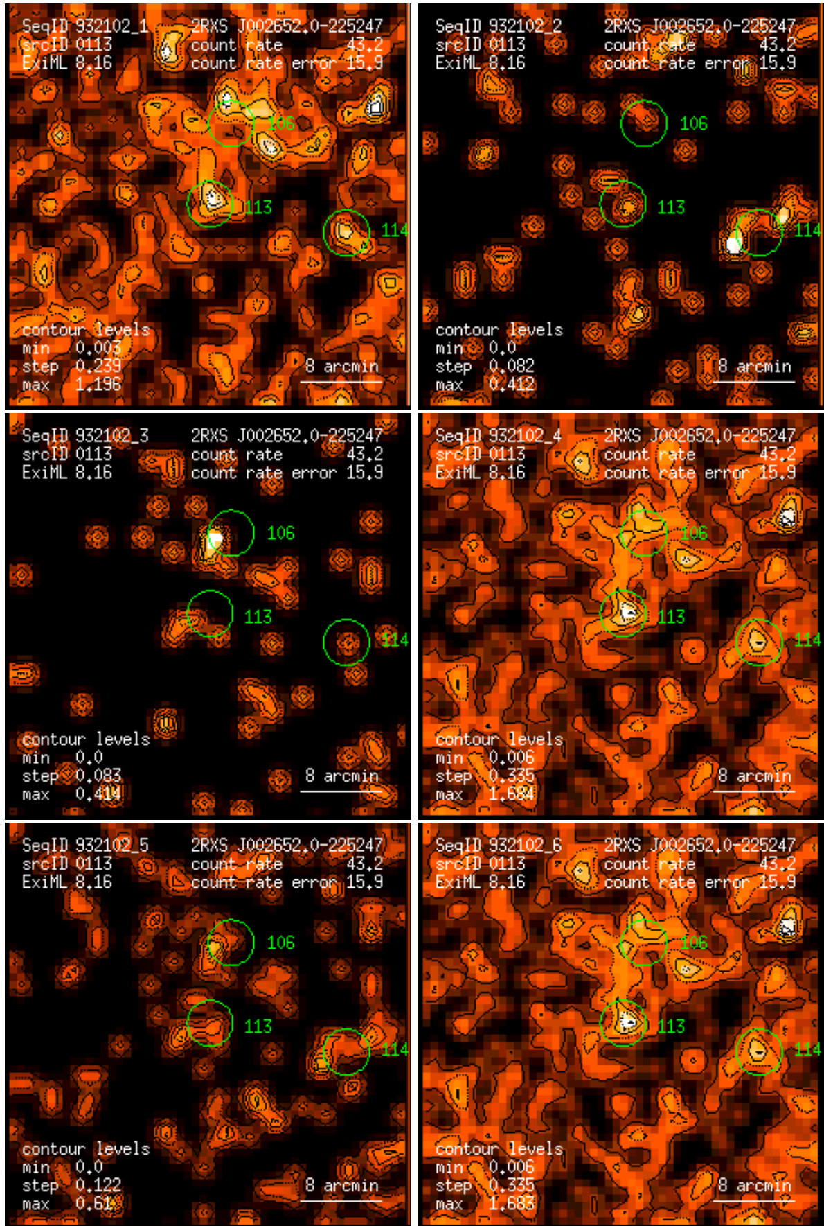
Figure 113: RASS 932102: detection 0113: band rate images, Gaussian filter: (1) PSPC channels 11 – 41, (2) 52 – 90, (3) 91 – 201, (4) 11 – 235, (5) 52 – 201, (6) 11 – 201. Broad band rates in counts/ks. Band rate contour levels in counts/ks/arcmin 2 .
