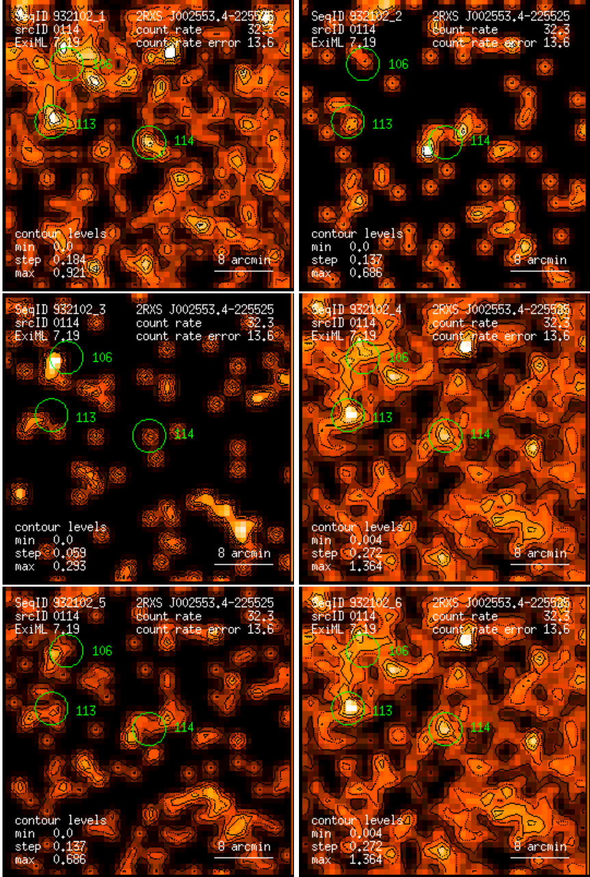
Figure 114: RASS 932102: detection 0114: band rate images, Gaussian filter: (1) PSPC channels 11 – 41, (2) 52 – 90, (3) 91 – 201, (4) 11 – 235, (5) 52 – 201, (6) 11 – 201. Broad band rates in counts/ks. Band rate contour levels in counts/ks/arcmin 2 .
