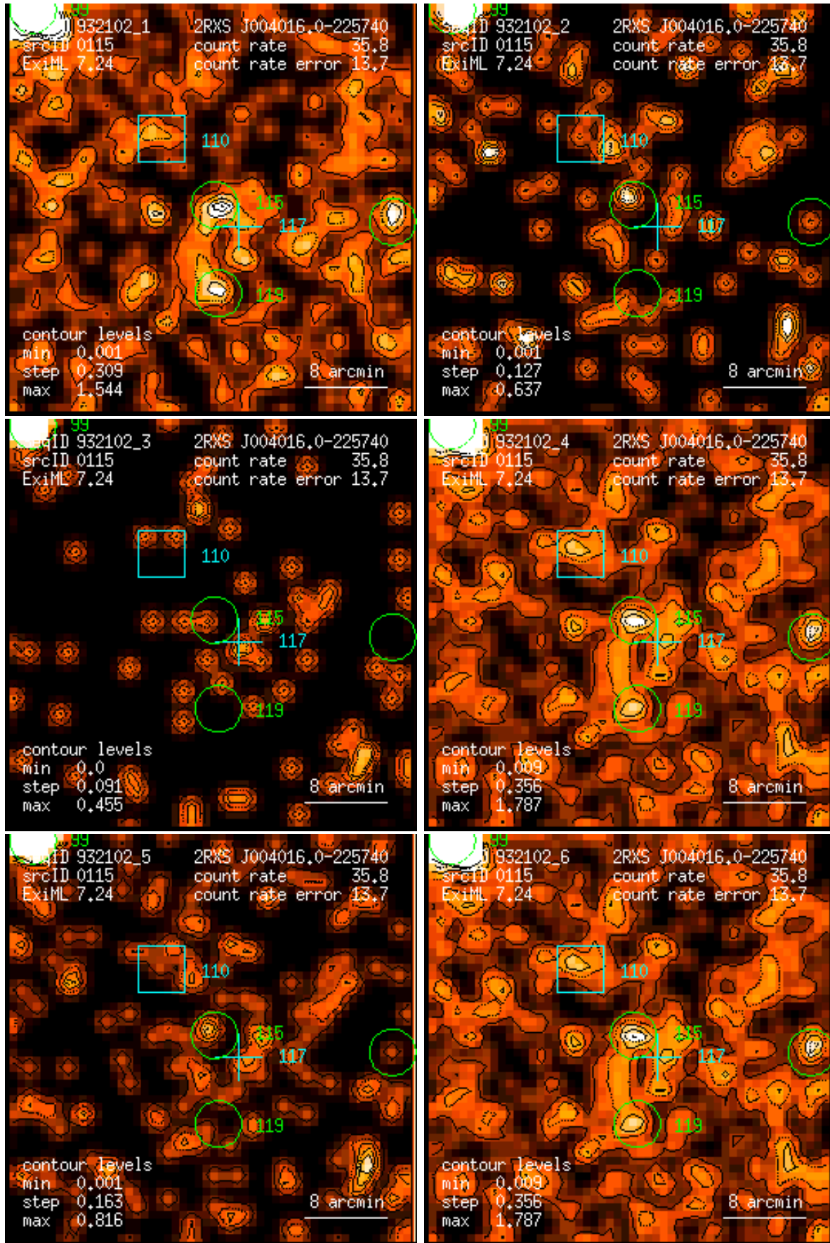
Figure 115: RASS 932102: detection 0115: band rate images, Gaussian filter: (1) PSPC channels 11 – 41, (2) 52 – 90, (3) 91 – 201, (4) 11 – 235, (5) 52 – 201, (6) 11 – 201. Broad band rates in counts/ks. Band rate contour levels in counts/ks/arcmin 2 .
