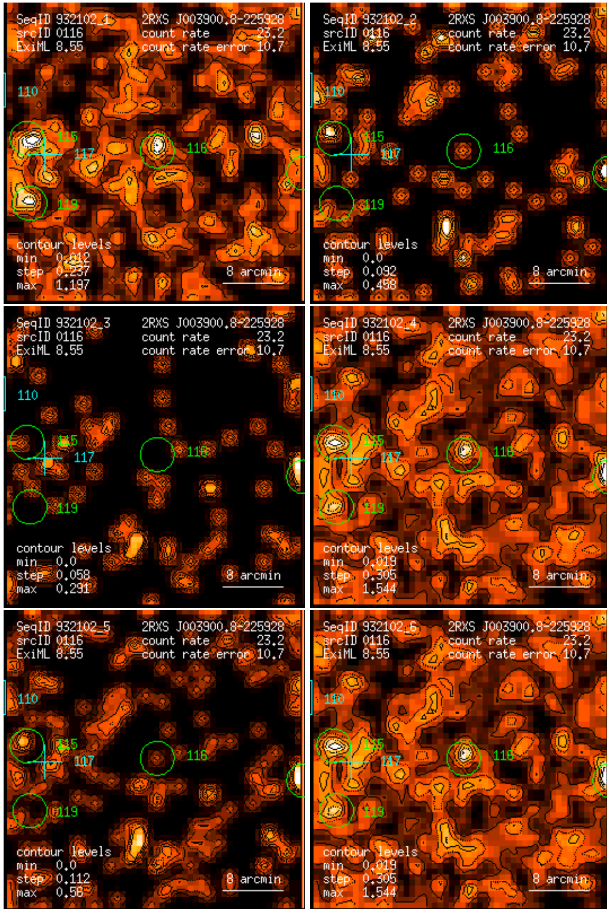
Figure 116: RASS 932102: detection 0116: band rate images, Gaussian filter: (1) PSPC channels 11 – 41, (2) 52 – 90, (3) 91 – 201, (4) 11 – 235, (5) 52 – 201, (6) 11 – 201. Broad band rates in counts/ks. Band rate contour levels in counts/ks/arcmin 2 .
