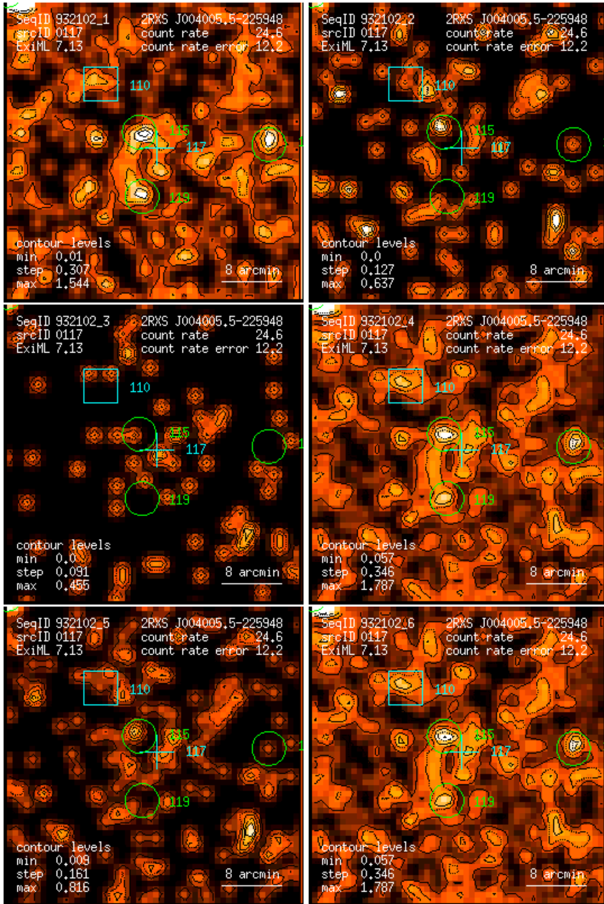
Figure 117: RASS 932102: detection 0117: band rate images, Gaussian filter: (1) PSPC channels 11 – 41, (2) 52 – 90, (3) 91 – 201, (4) 11 – 235, (5) 52 – 201, (6) 11 – 201. Broad band rates in counts/ks. Band rate contour levels in counts/ks/arcmin 2 .
