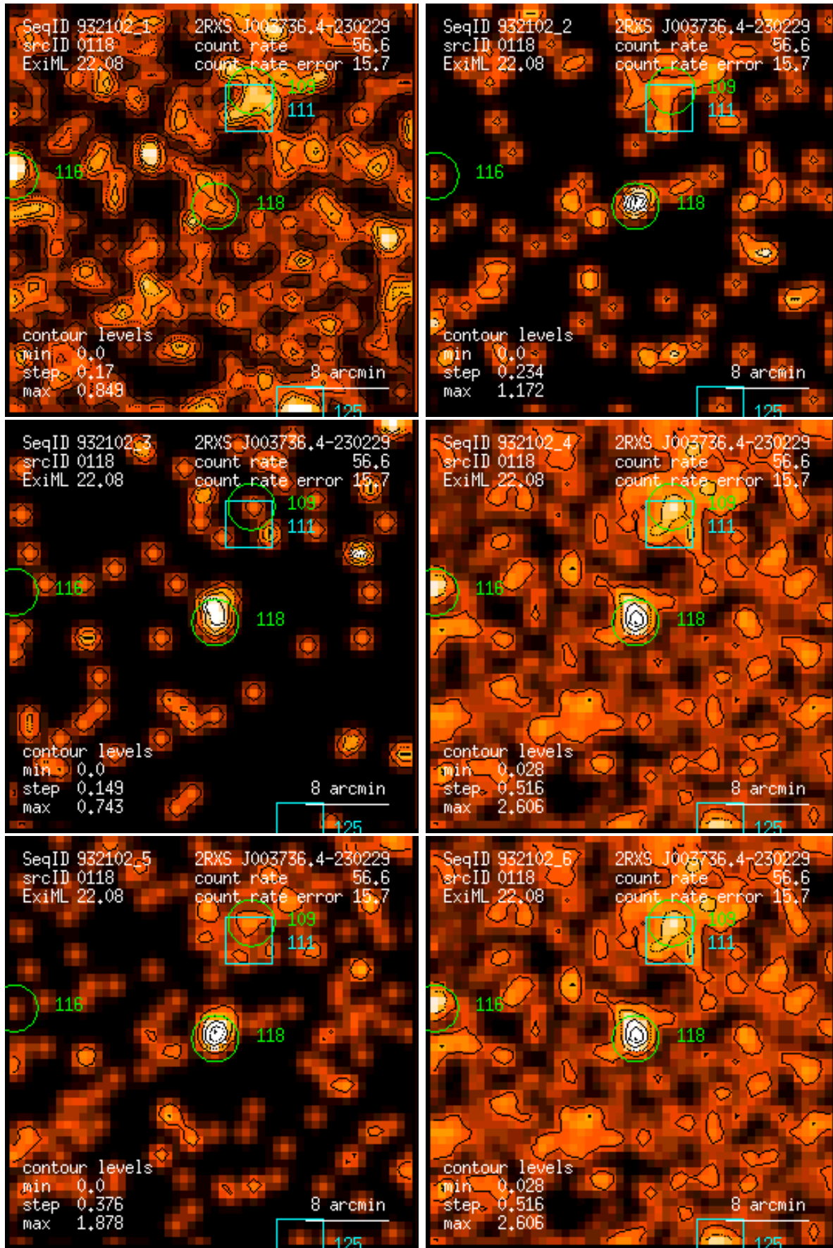
Figure 118: RASS 932102: detection 0118: band rate images, Gaussian filter: (1) PSPC channels 11 – 41, (2) 52 – 90, (3) 91 – 201, (4) 11 – 235, (5) 52 – 201, (6) 11 – 201. Broad band rates in counts/ks. Band rate contour levels in counts/ks/arcmin 2 .
