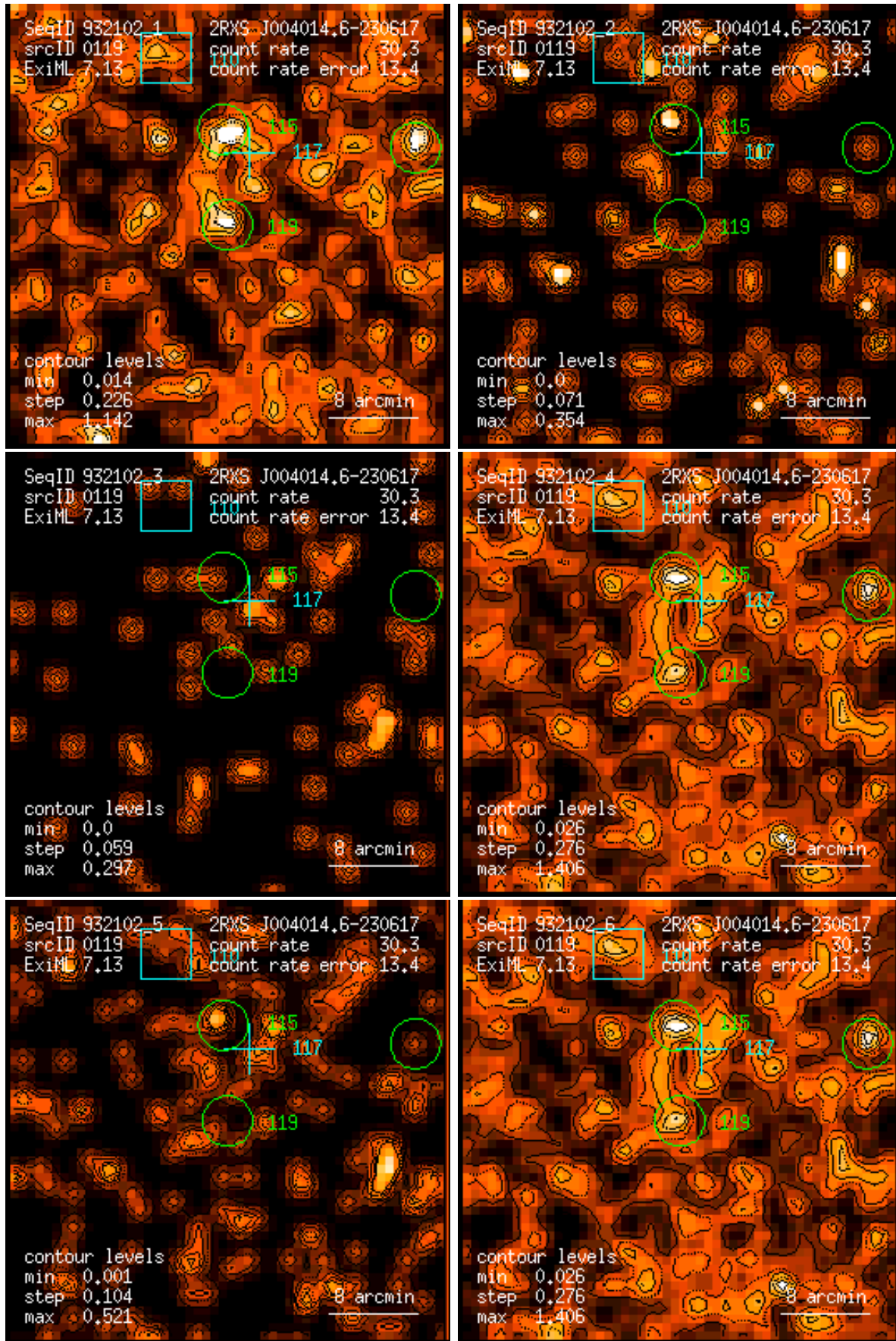
Figure 119: RASS 932102: detection 0119: band rate images, Gaussian filter: (1) PSPC channels 11 – 41, (2) 52 – 90, (3) 91 – 201, (4) 11 – 235, (5) 52 – 201, (6) 11 – 201. Broad band rates in counts/ks. Band rate contour levels in counts/ks/arcmin 2 .
