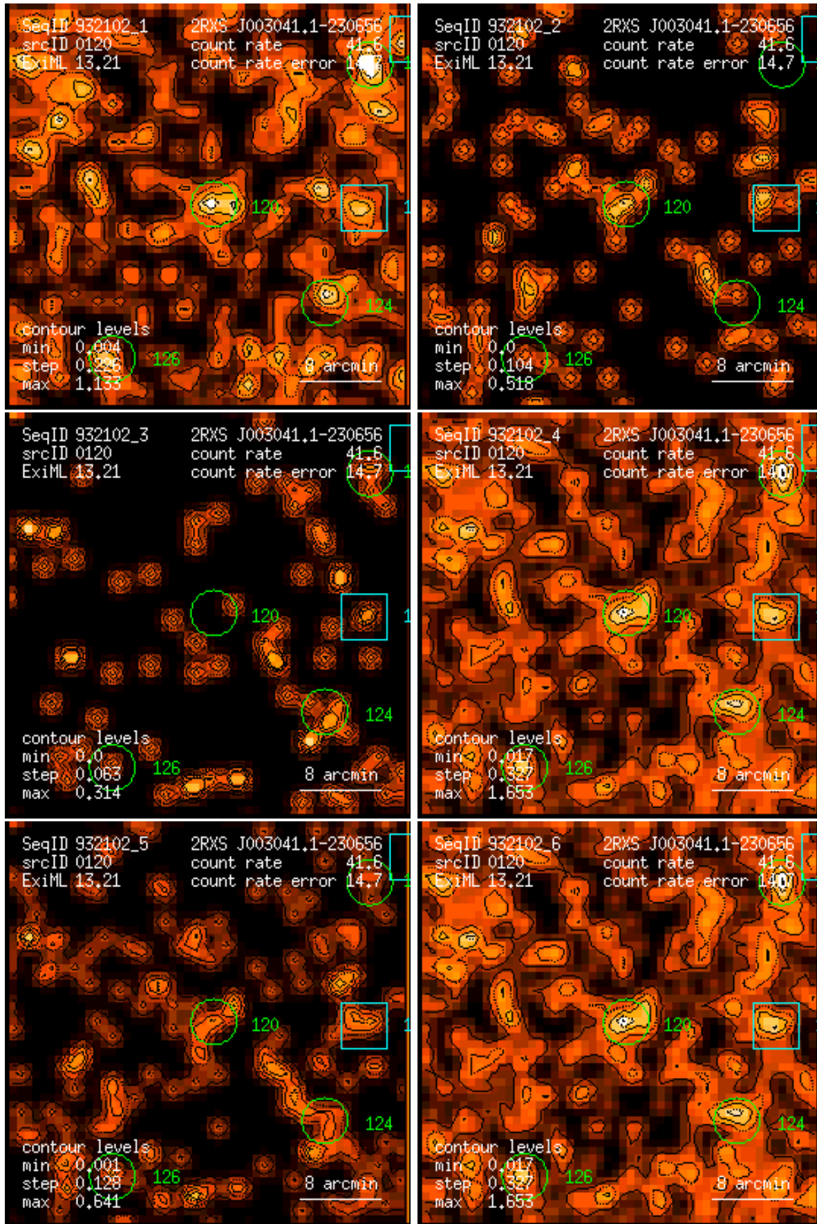
Figure 120: RASS 932102: detection 0120: band rate images, Gaussian filter: (1) PSPC channels 11 – 41, (2) 52 – 90, (3) 91 – 201, (4) 11 – 235, (5) 52 – 201, (6) 11 – 201. Broad band rates in counts/ks. Band rate contour levels in counts/ks/arcmin 2 .
