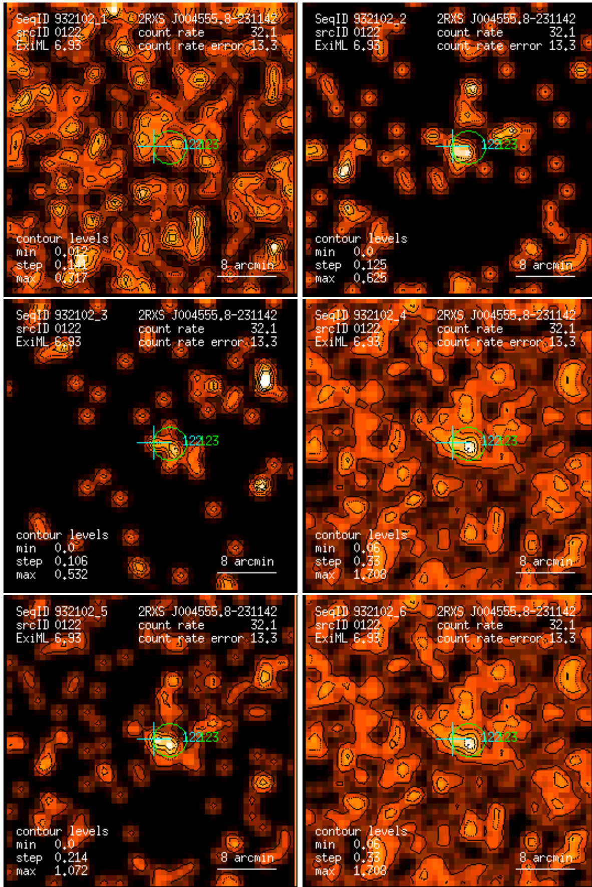
Figure 122: RASS 932102: detection 0122: band rate images, Gaussian filter: (1) PSPC channels 11 – 41, (2) 52 – 90, (3) 91 – 201, (4) 11 – 235, (5) 52 – 201, (6) 11 – 201. Broad band rates in counts/ks. Band rate contour levels in counts/ks/arcmin 2 .
